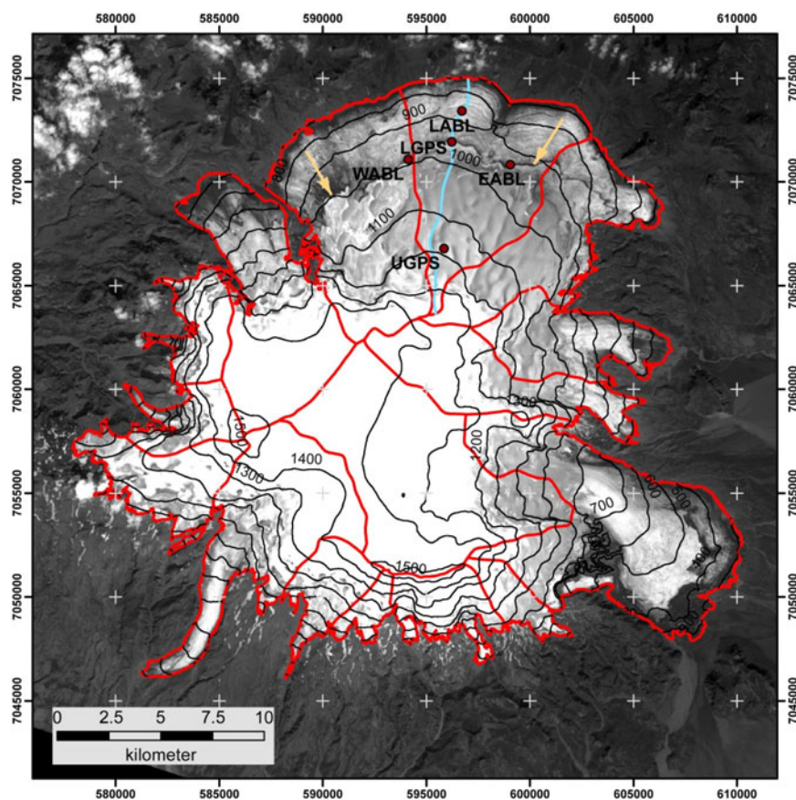
Fig. 1. Landsat 8 satellite image of Mýrdalsjökull Ice Cap from 12 August 2014. The red curve displays the glacier boundary and the principal drainage units, including debris-covered glacier areas. On the northern lobe, Sléttjökull is composed of the three northernmost sub-basins. The locations of field measurements in 2013/14 are indicated, as well as the flowline profile (blue). Arrows indicate the position of the tephra layer outcrop. Contours are based on a DEM of Iceland compiled by Hans H. Hansen, Fixlanda ehf., Iceland (Lidar data source: Icelandic Meteorological Office and Institute of Earth Sciences, University of Iceland, 2013; DEMs of Icelandic glaciers (dataset)).
