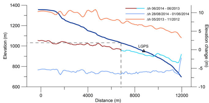
Fig. 6. Surface elevation change (right axis) derived from TanDEM-X imagery for the time span June 2013–June 2014 (light blue/red curves), winter 2012/13 (November until May, orange curve) and summer 2014 (1 June–28 August, blue curve). The surface elevation along the flowline from the ice margin to the caldera rim is shown as dark blue curve (left axis).
