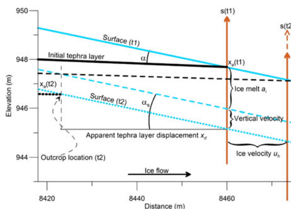
Fig. 3. Schematic diagram of the components influencing the apparent tephra layer displacement, based on the field observations at the tephra outcrop of the 1918 eruption on Sléttjökull. The horizontal axis originates at the ice divide and is oriented along the ice flow. The light blue line represents the glacier surface at time t_1 , with the layer outcrop at x_a(t_1) . The emergence angle of the tephra layer with respect to the surface is \alpha and the surface inclination from the horizontal is \alpha_s . The stake s(t_1) (and the layer outcrop x_a(t_1) ) are moved by ice transport to s(t_2) , while the surface is lowered by ice melt to the dashed blue line during the same time span. Due to this removal of ice, the outcrop position is shifted to the location x_a(t_2) and the tephra layer apparently moves upstream. The vertical ice velocity at the surface lowers the surface (dashed blue line) to the position of the dotted blue line, while x_a(t_2) does not change its horizontal position.
