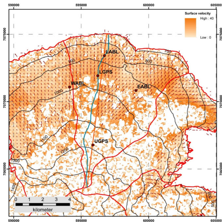
Fig. 5. Surface velocities ( \text{m a}^{-1} ) from 10 September 2011 to 01 August 2012, derived by feature tracking from Rapid Eye imagery. Velocity vectors are only shown in areas with reliable and dense feature tracking results. The blue curve represents the true flowline, while the orange line is the idealized flowline for modelling purposes.
