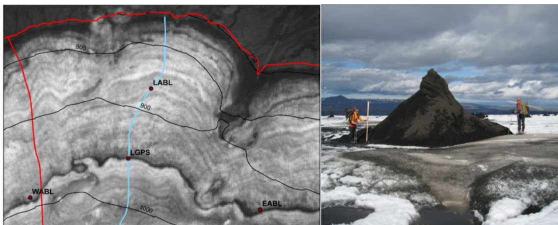
Fig. 2. Left: Tephra layer outcrop of the 1918 Katla eruption in the region of the field work at Sléttjökull (at the station LGPS). Right: Ash cone downstream of the tephra layer outcrop (Photo: J. Jaenicke, 2013).
