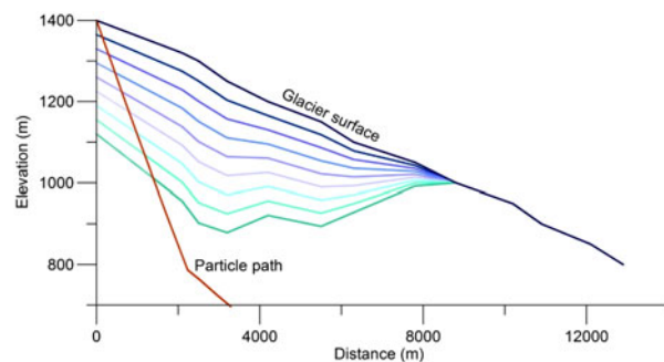
Fig. 4. Simple modelling of the englacial tephra layer geometry from the eruption in 1918 in 10 year steps, calculated by a generalized flowline approach (Eqn (3)) and hypothetical steady-state conditions. The tephra layer is buried gradually in the accumulation zone (coloured curves from blue to green) beneath the steady glacier surface (black) and it emerges at the surface downstream of the equilibrium line, where it will be eroded by rain and ice melt. The red curve shows the path through the ice cap of a tephra particle deposited at the uppermost location of our flowline model through the ice cap.
