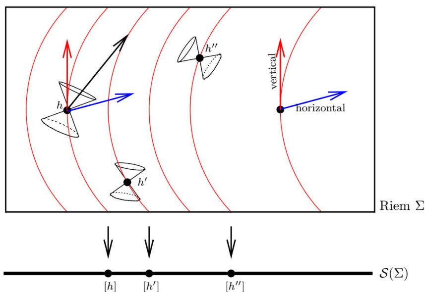
Figure 5.2: The space \text{Riem } \Sigma , fibred by the orbits of \text{Diff } \Sigma (curved vertical lines). Tangent directions to these orbits are called “vertical”, the G -orthogonal directions “horizontal”. Horizontal and vertical directions intersect whenever the “hyper-lightcone” touches the vertical directions, as in point h' . At h , h' , and h'' the vertical direction is depicted as time-, light-, and space-like respectively. Hence [h'] corresponds to a transition point where the signature of the metric in superspace changes. From [4]
