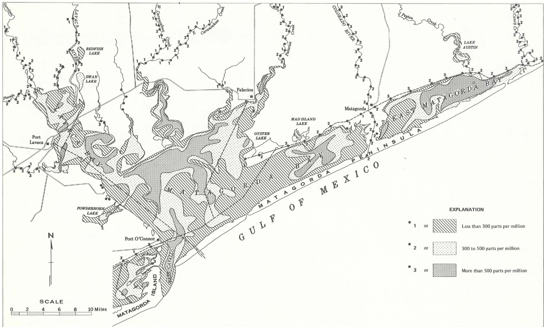
Figure 9. Barium distribution map.
