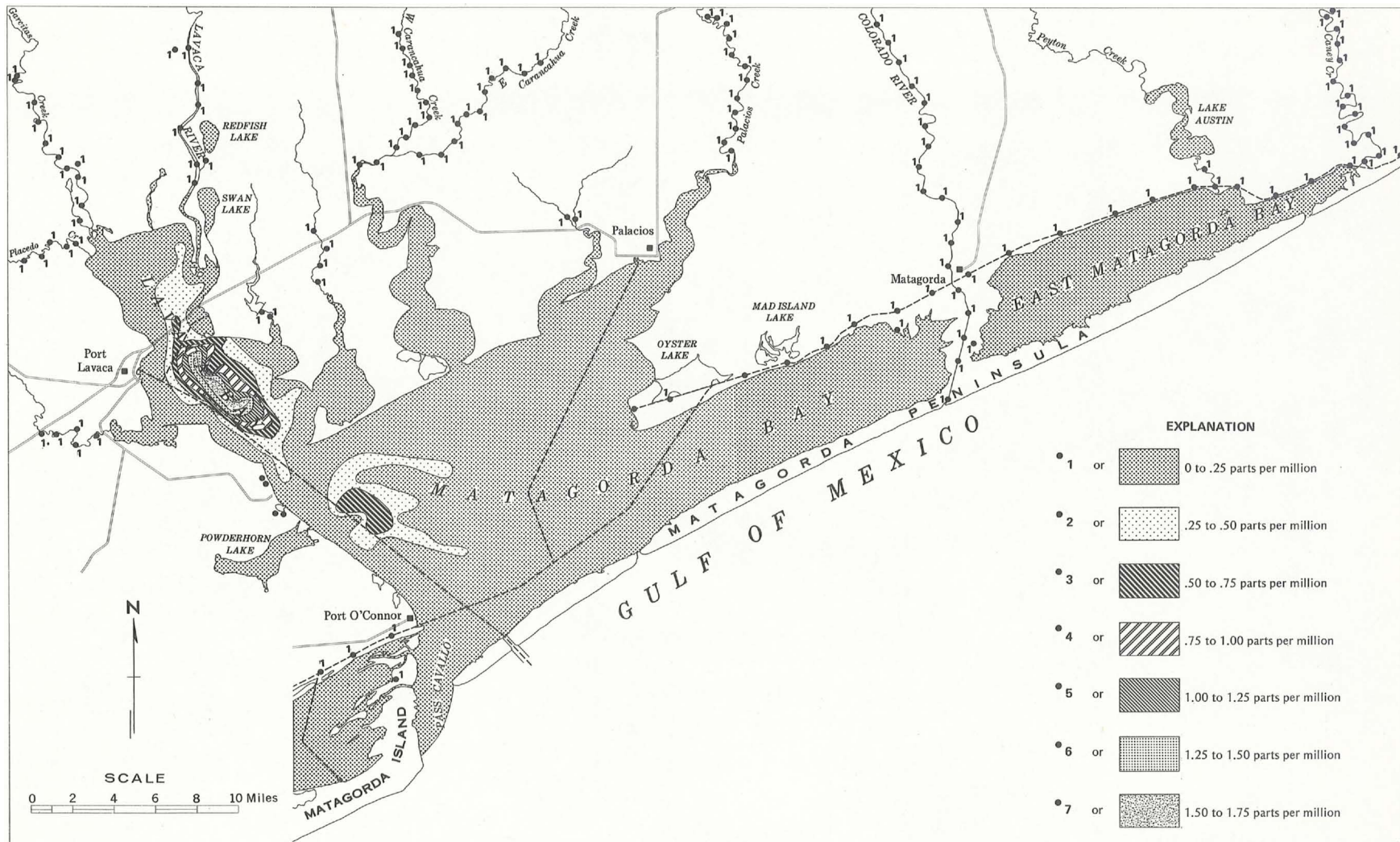
Figure 16. Mercury distribution map.
