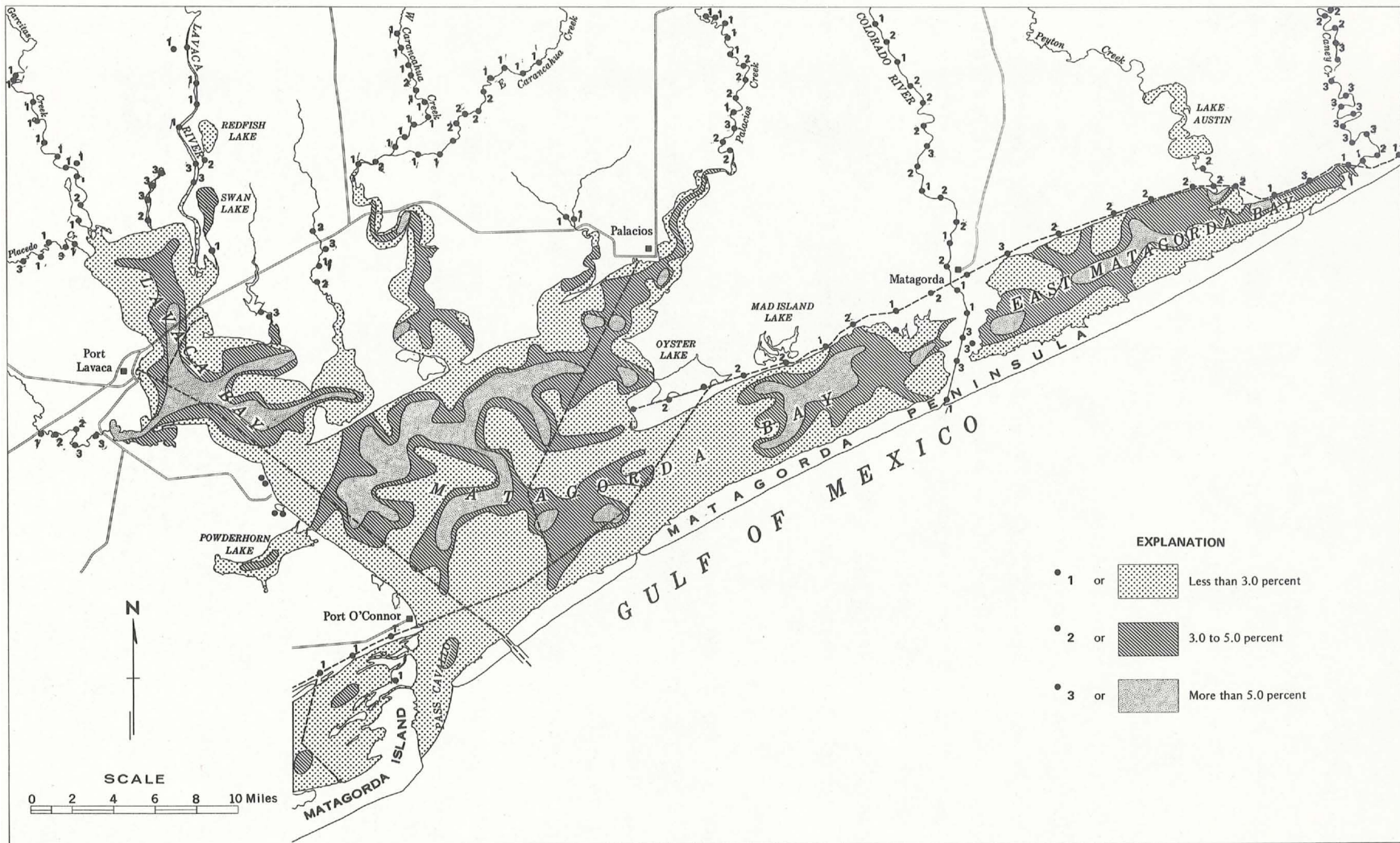
Figure 15. Iron distribution map.
