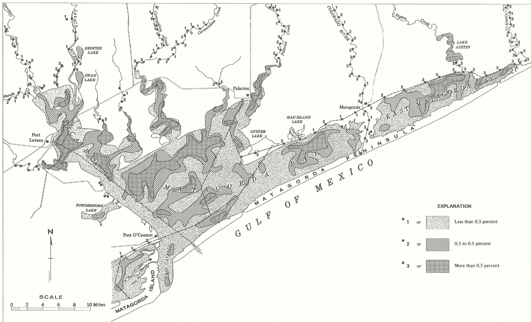
Figure 24. Titanium distribution map.
