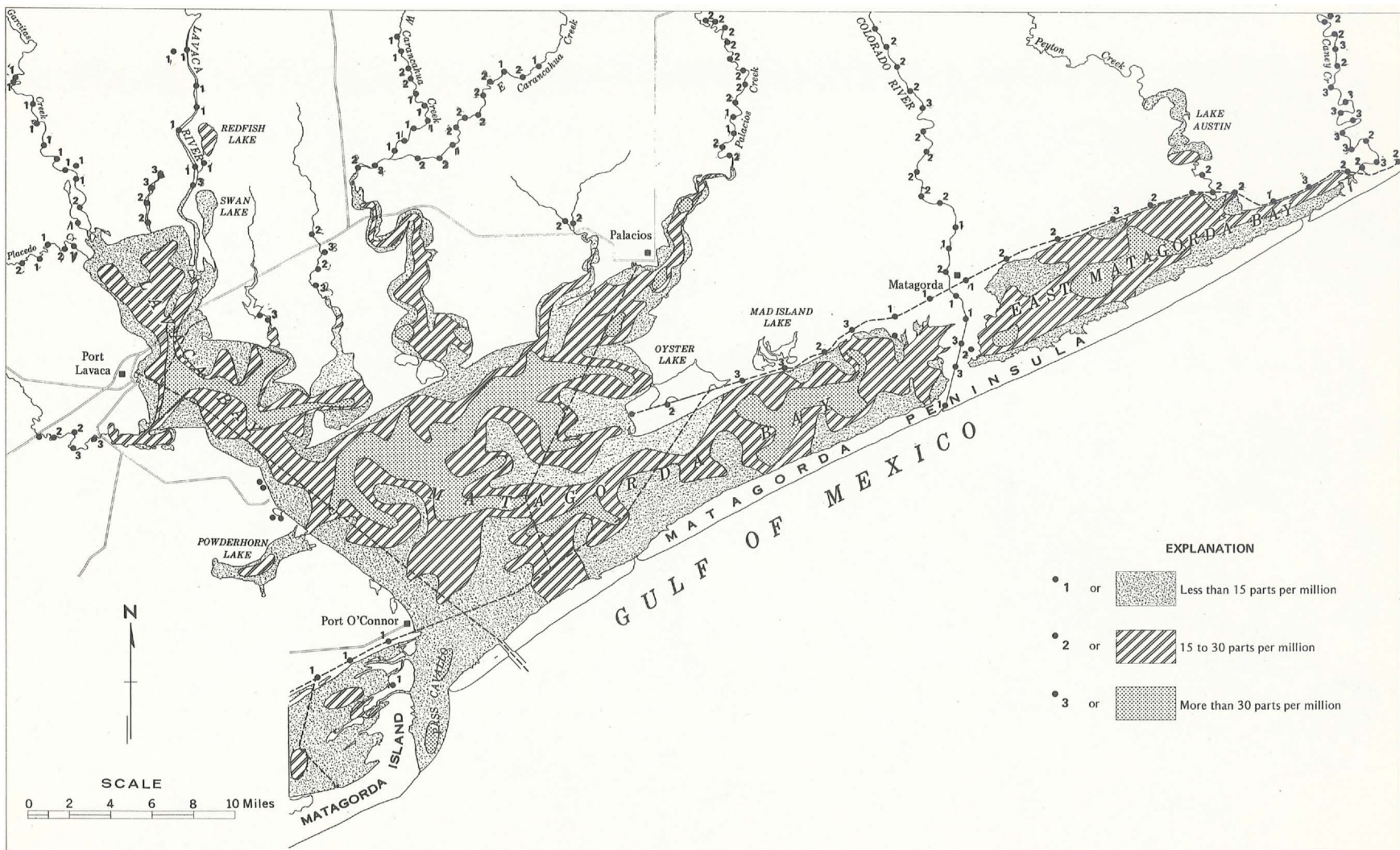
Figure 21. Nickel distribution map.
