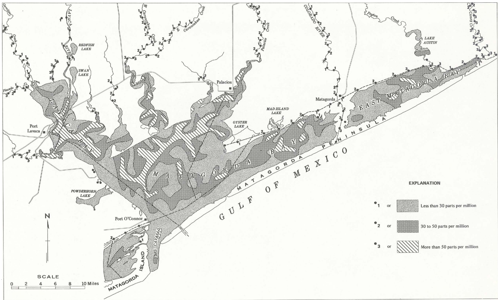
Figure 17. Lanthanum distribution map.
