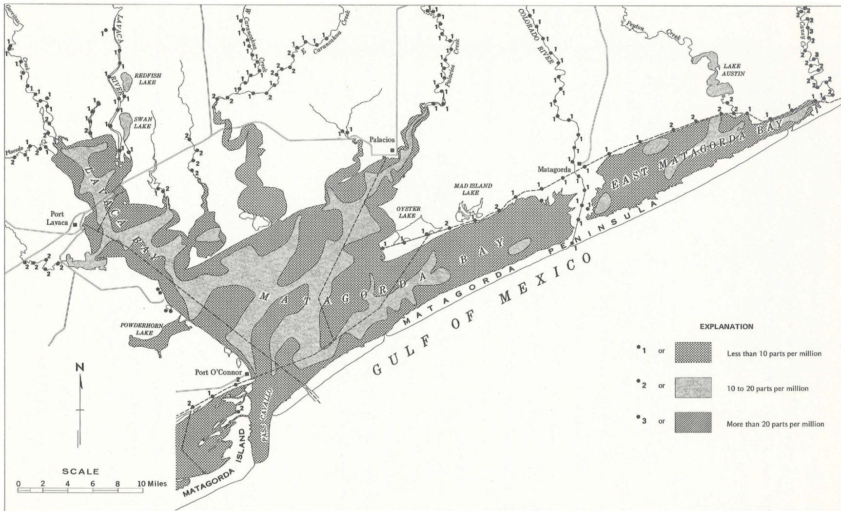
Figure 20. Niobium distribution map.
