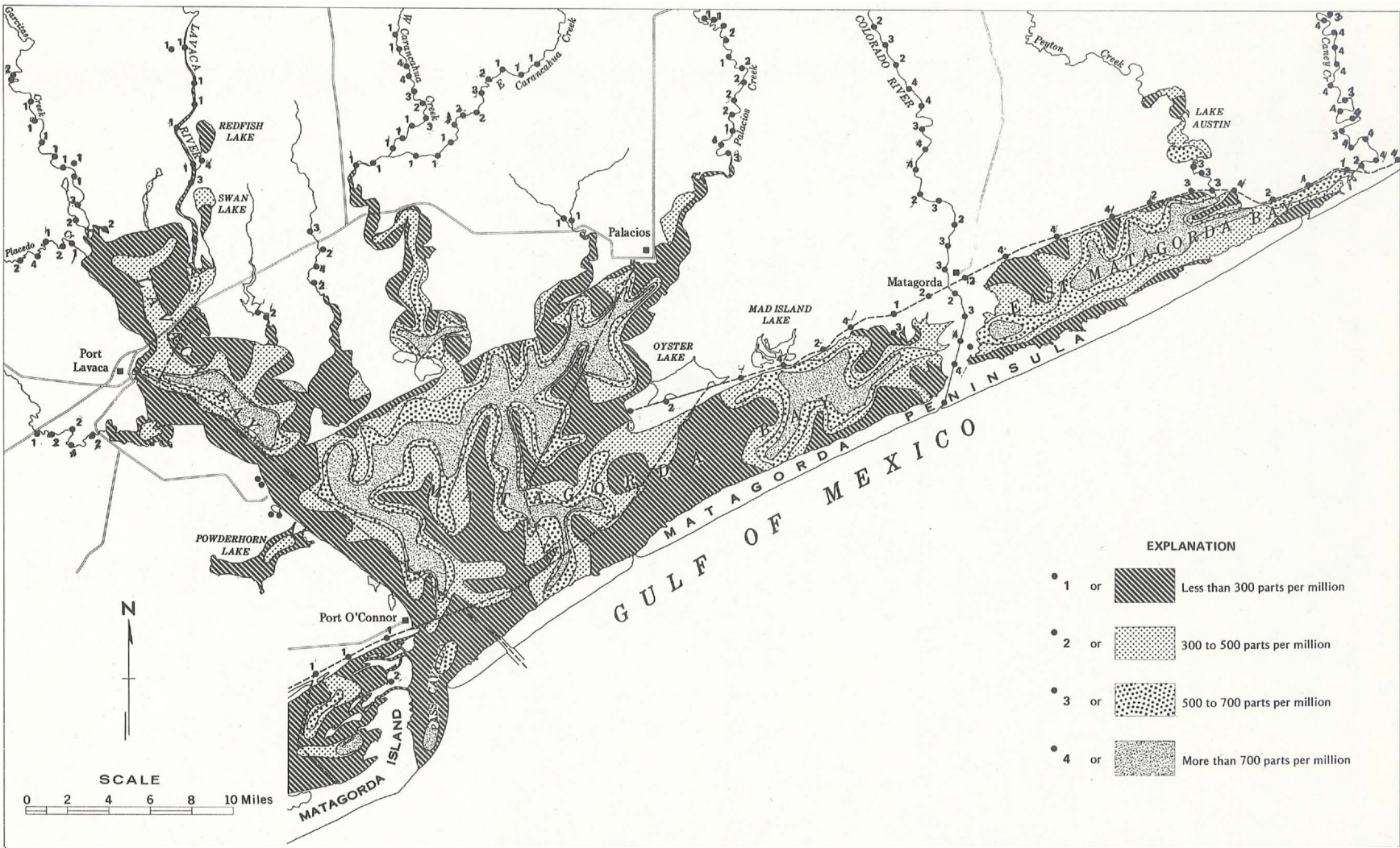
Figure 19. Manganese distribution map.
