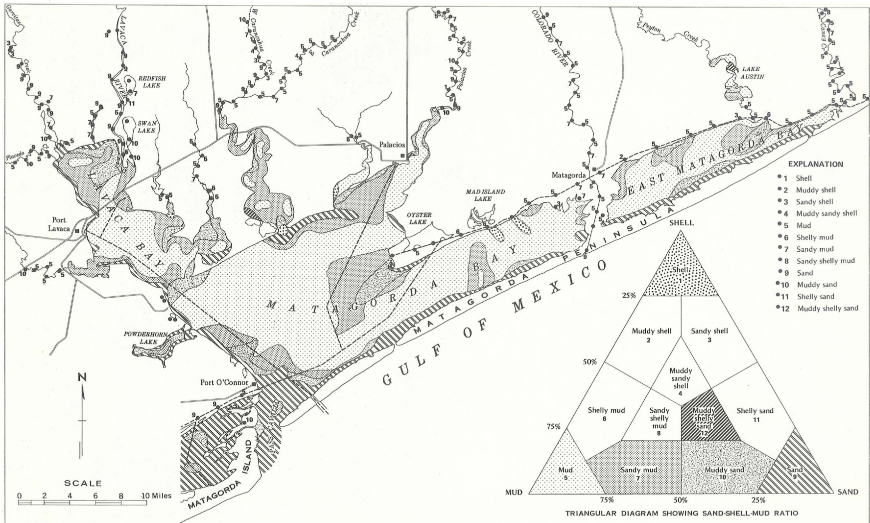
Figure 6. Sediment distribution map.
