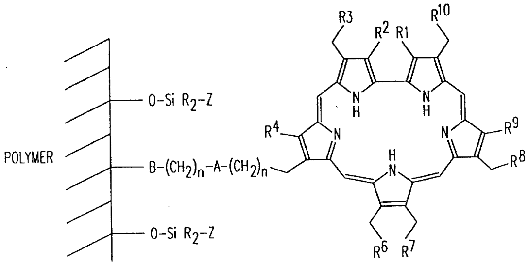
GENERAL STRUCTURE VII
