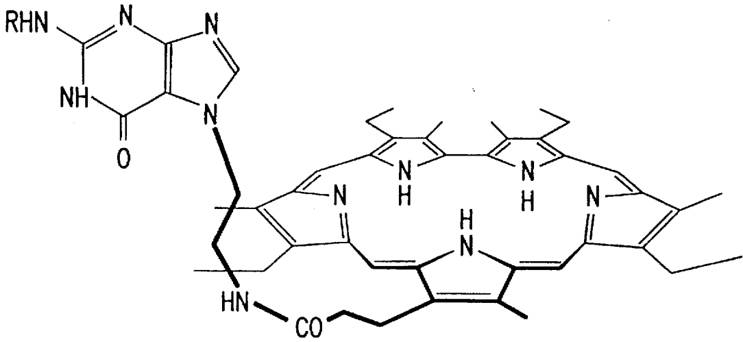
STRUCTURE 11 R = Bz
