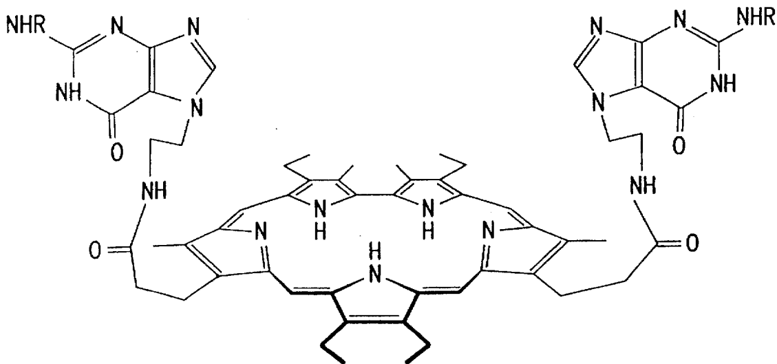
STRUCTURE 17 R = Bz
