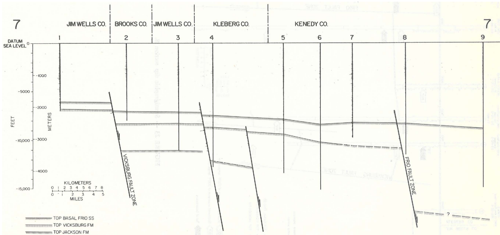
FIGURE 22 — Structure section 7.
