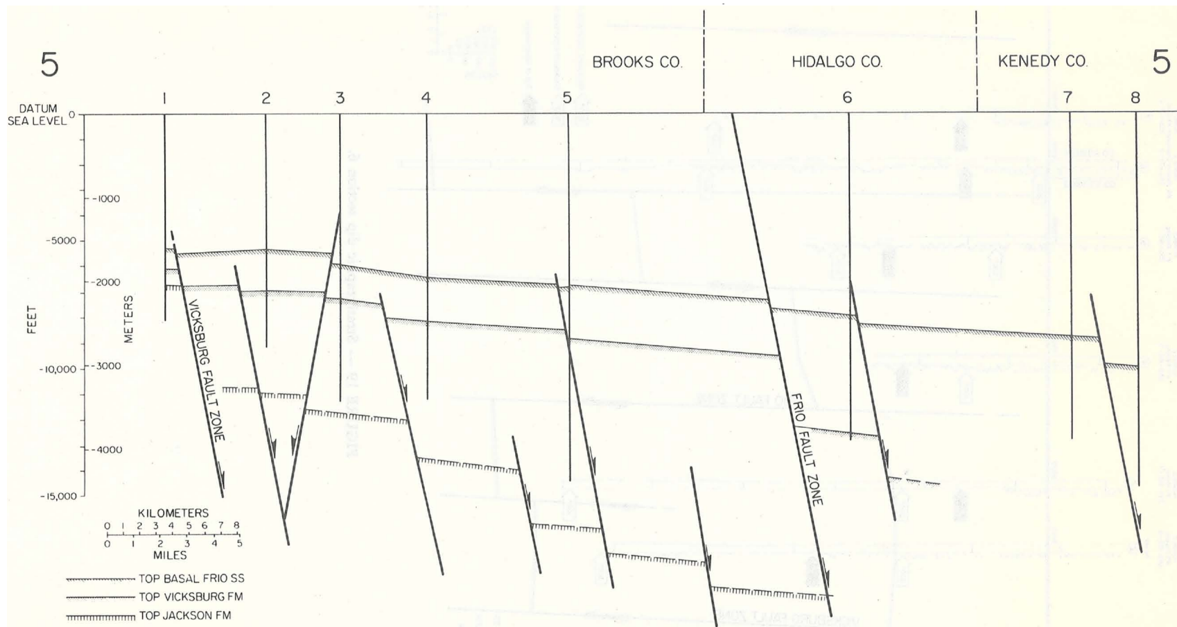
FIGURE 18 — Structure section 5.
