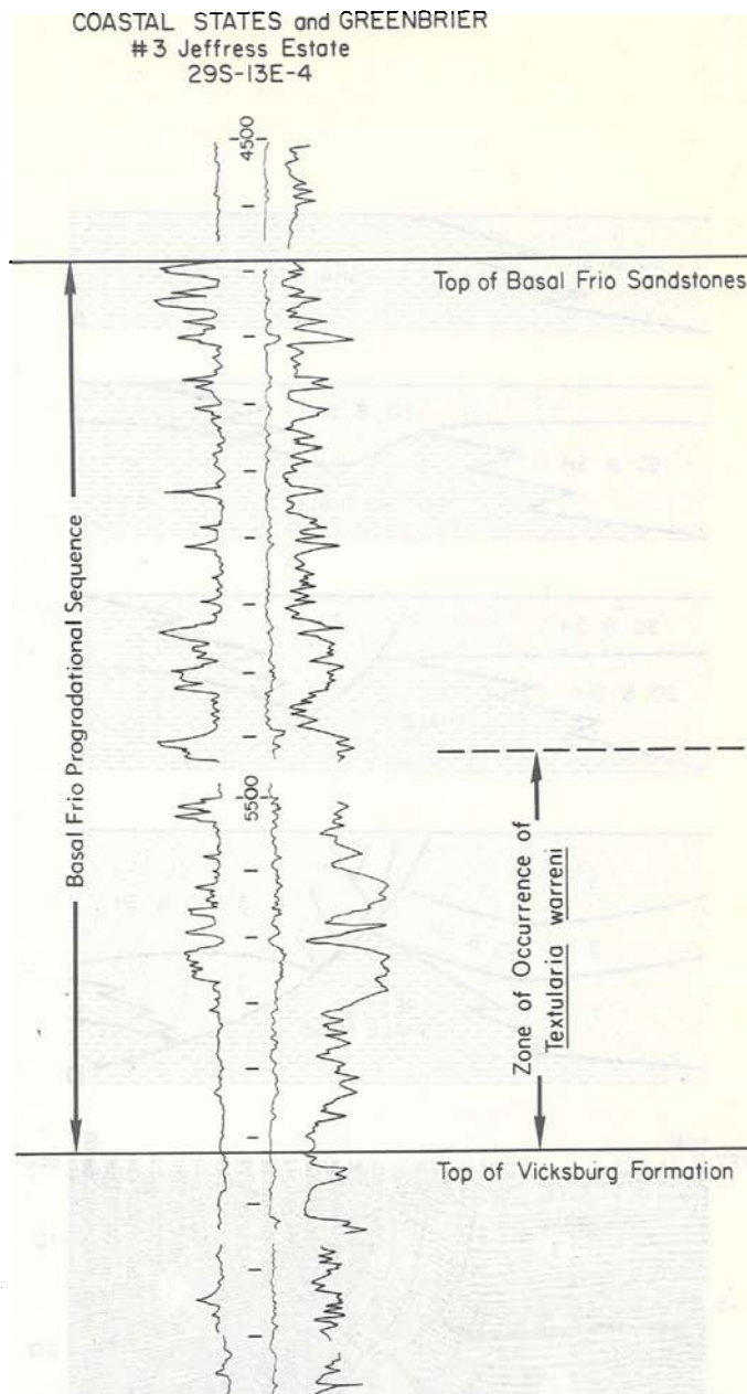
FIGURE 7 — Electrical log showing contact between Vicksburg and basal Frio sandstones. Zone of occurrence of Textularia warreni is in the lower part of the basal Frio progradational sequence.
