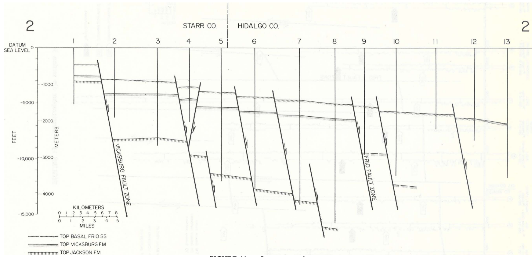
FIGURE 12 -- Structure section 2.
