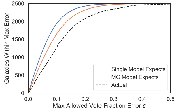
(b) Calibration for ‘Bar’
