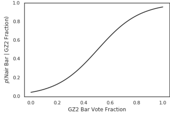
Figure A3. The rescaling function used to map GZ2 vote fractions to p(\text{Nair Bar}|\text{GZ2 Fraction}) , estimated via logistic regression. This rescaling function is also used (without modification) to map Bayesian CNN GZ2 vote fraction predictions to p(\text{Nair Bar}|\text{BCNN-predicted GZ2 Fraction})
