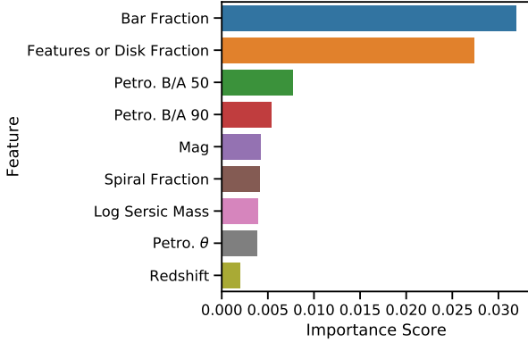
Figure 6. Relative importance of morphological (Features or Disk, Bar, Spiral) and non-morphological (Petro B/A, Mag, etc.) features for BCNN performance. Morphology fractions are the (human-reported) \frac{k}{N} values from Galaxy Zoo 2. Petro B/A 50 and Petro B/A 90 measure the axial ratios at 50% and 90% of the half-light radius. Mag is the estimated B magnitude. Sersic mass is the approximate stellar mass, estimated from the single-component Sersic fit flux. Petro \theta is the ( r -band) Petrosian radius. Redshift is measured spectroscopically. The effect of each component is additive and independent; for example, the measured effect of spiral features does not include the effect of being featured in general. BCNN performance varies much less from the effect of non-morphological features than from morphological features.
