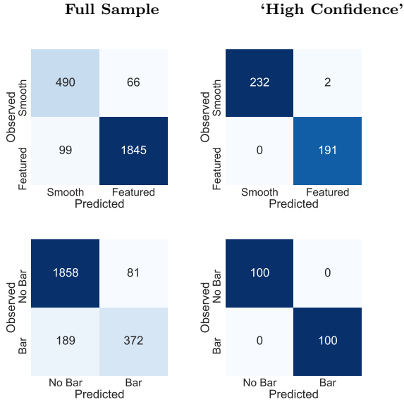
Figure 10. Confusion matrices for ‘Smooth or Featured’ (upper row) and ‘Bar’ (lower row) questions. For comparison to K+18, we also include confusion matrices for the most confident predictions (right column). Following K+18, we include the most confident \sim 7.7\% of spirals and \sim 9.3\% of ellipticals (upper right). Of the two galaxies where humans select ‘Smooth’ ( \frac{k}{N} > 0.5 ) and the model selects ‘Featured’ ( \hat{p} < 0.5 ), one is an ongoing smooth/featured major merger and one is smooth with an imaging artifact. Generalising (K+18 do not consider bars), we also show the most confident \sim 8\% of barred and unbarred galaxies. We achieve perfect classification for ‘Bar’.
