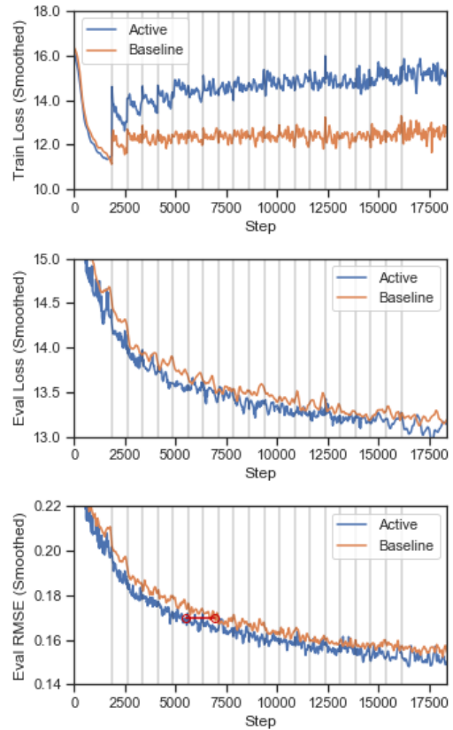
Figure 12. As with 11, but for the ‘Bar’ active learning simulations. Again, active learning leads to a clear improvement in evaluation performance and a dramatically higher training loss (indicating challenging galaxies are being selected). We annotate in red where each model achieves the maximal relative RMSE improvement, highlighting the reduction in newly-labelled galaxies required (vertical bars = 256 new galaxies).
