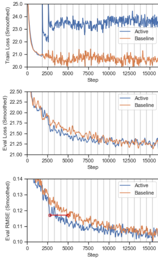
Figure 11. Training loss (upper), evaluation loss (middle), and RMSE (lower) of model performance on ‘Smooth or Featured’ during active learning simulations, by iteration (set of new galaxies). Vertical bars denote new iterations, where new galaxies are acquired and added to the training set. Prior to 2000 training iterations, both the random selection (baseline) models and active learning models train on only the initial random training set of 256 galaxies, and hence show similar performance. Around 2000 to 3500 iterations, after acquiring 128-256 additional galaxies, the active learning model shows a clear improvement in evaluation performance over the baseline model. We annotate in red where each model achieves the maximal relative RMSE improvement, highlighting the reduction in newly-labelled galaxies required (vertical bars = 128 new galaxies). Note that active learning leads to a dramatically higher training loss, indicating that more challenging galaxies are being identified as informative and added to the training set.
