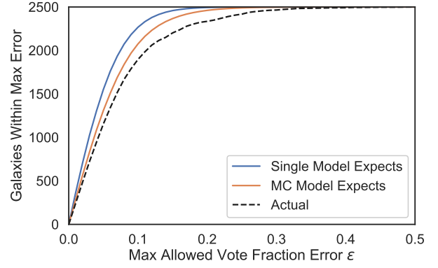
(a) Calibration for ‘Smooth or Featured’
