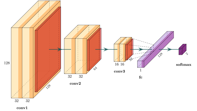
Figure 3. The CNN architecture used throughout. The input image, after applying augmentations (Section 2.5.3), is of dimension 128 \times 128 \times 1 . The first pair of convolutional layers are each of dimension 128 \times 128 \times 32 with 3 \times 3 kernels. We then max-pool down to a second pair of convolutional layers of dimension 64 \times 64 \times 32 with 3 \times 3 kernels, then again to a final pair of dimension 32 \times 32 \times 16 with 3 \times 3 kernels. We finish with a 128-neuron linear dense layer and a 2-neuron softmax dense layer.
