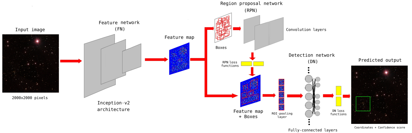
Figure 1. High-level overview of the architecture for the Faster-RCNN algorithm which contains the Feature Network, Region Proposal Network and Detection Network. The output from each network is used as the input for the next network. This architecture is similar to the system demonstrated in Figure 2 from Ren et al. (2015). The full details of the INCEPTION-V2 architecture can be found in Ren et al. (2018). For simplicity, the layers in the INCEPTION-V2 architecture and the FN are not displayed fully, and we do not show the ReLU activation layers in any of the networks. The RPN and the DN loss functions are active during the training phase, but they are replaced by a softmax classifier layer (Nwankpa et al. 2018) in the testing phase.
