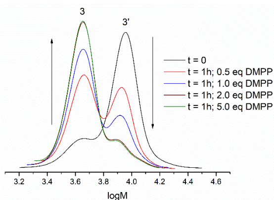
Fig. 2 SEC (THF) chromatograms at t = 1h, demonstrating the in-situ reduction of 3' to 3 in the presence of increasing amounts of DMPP.
