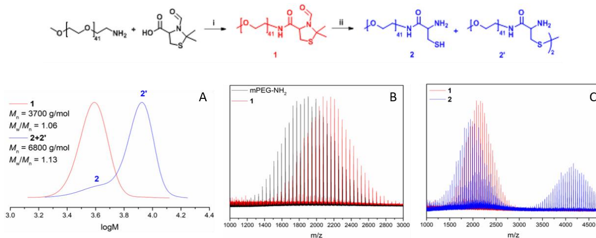
Fig. 1 Synthesis of terminal cysteine-functional PEG. Two step synthesis, i) CDI, CHCl 3 , RT, ii) HCl (0.5 M), 70 °C; (A) SEC traces, DMF; (B, C) MALDI spectra of the protected ( 1 ) and deprotected ( 2 , 2' ) compound.
