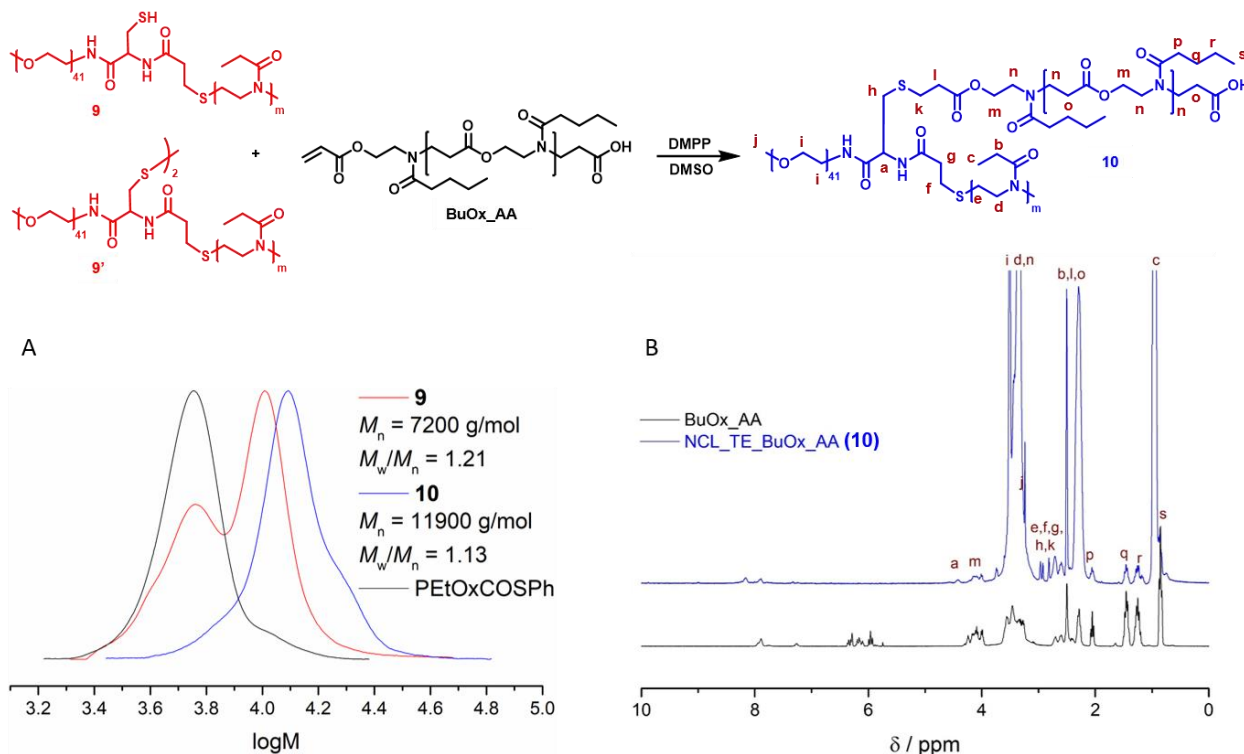
Fig. 5 Synthesis of 3-arm miktoarm star terpolymer \mu -(PEG,PETox,NPAE) ( 10 ). Thiol-Michael addition of 9,9' and oligo(BuOx-alt-AA) n A; (A) SEC traces and (B) 1 H NMR spectra.
