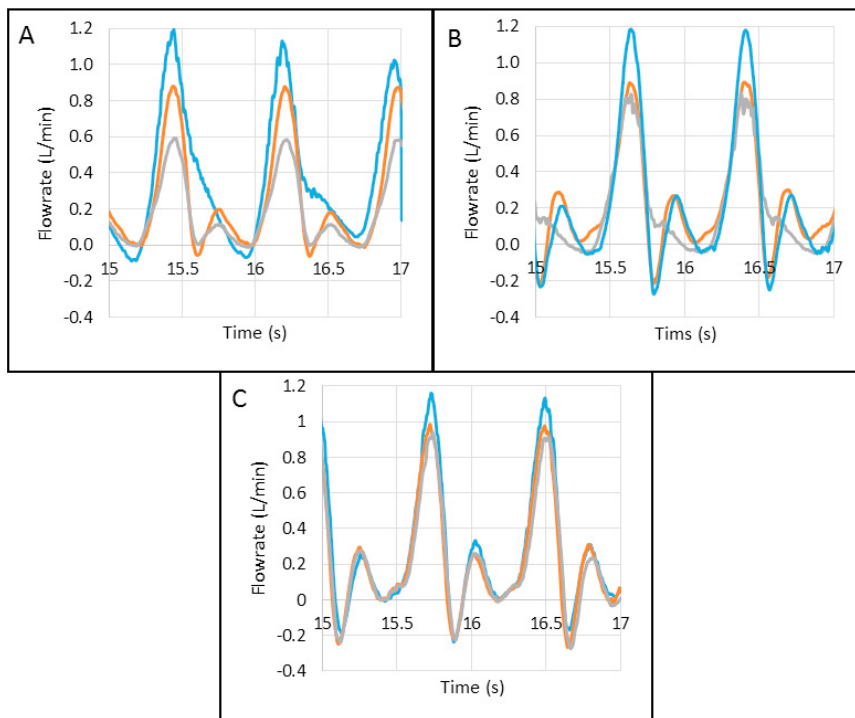
Fig. 5. Change in flowrate at A) 5mm, B) 50mm and C) 100mm (Blue=Healthy, Red=Palmaz, Green=Zigzag)
