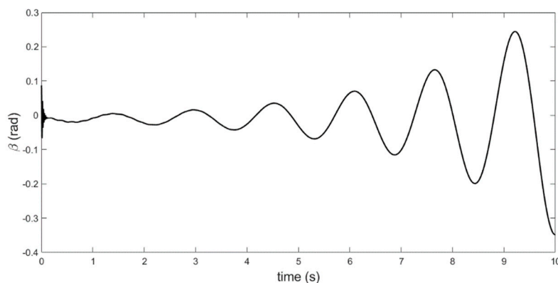
Figure 12. Time response of beta in upper speed of flutter (35 m/s).
