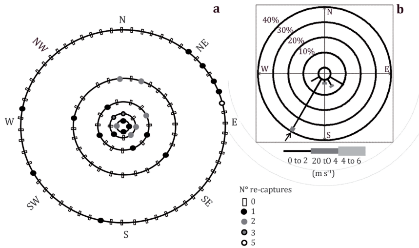
Figure 1. (a) Diagram of the field trial indicating the position of the 117 traps set at five distances (6, 12, 24, 48, and 96 m) from the central point where Liriomyza huidobrensis individuals were released. Different symbols indicate different number of re-captures (b) Circular histogram illustrating wind direction and speed during the experiment. Each ring represents the time proportion (%) of winds from different directions. The arrow indicates the prevailing wind direction.
