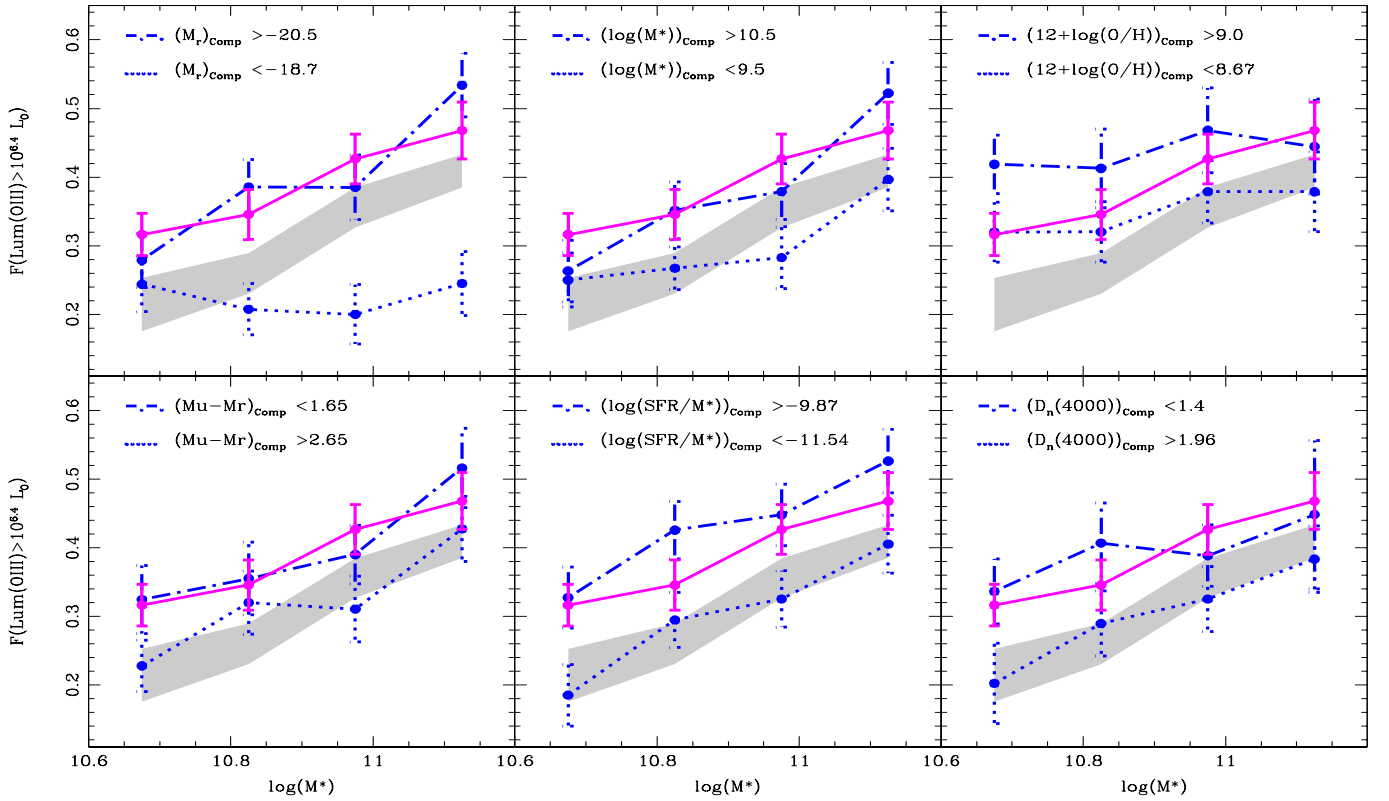
Fig. 9. Fraction of Lum[\text{OIII}] > 10^{6.4} L_{\odot} as a function of stellar mass, \log(M^*) , for barred AGN galaxies (solid lines) and AGNs in pairs with restrictions in the galaxy pair companion properties defined in the text (dotted and dot-dashed lines). The gray surfaces represent the control sample within uncertainties derived through the bootstrap resampling technique. Each bin for each sample contains a similar number of galaxies. The average number of galaxies in each bin is \approx 105 for BARRED-AGN, \approx 140 for CS and \approx 67 for AGN IN PAIRS with restrictions in the properties of the galaxy pair companion.
