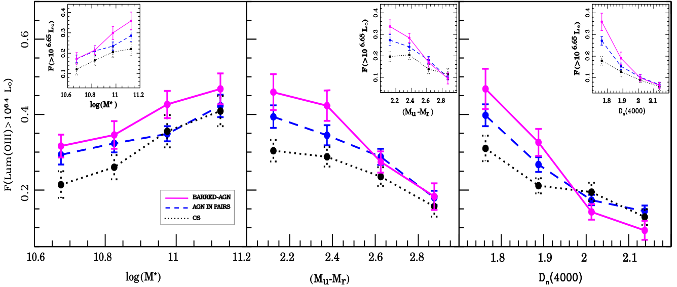
Fig. 5. Fraction of Lum[OIII] > 10^{6.4} L_{\odot} as a function of stellar mass, (M_u - M_r) color, and D_n(4000) parameter ( left , middle and right panels, respectively), for barred AGN galaxies (solid lines), AGN in pair systems (dashed lines), and unbarred AGN in the control sample (dotted lines). Each bin for each sample contains a similar number of galaxies. The number average of galaxies in each bin is \approx 105 for BARRED-AGN \approx 310 for AGN IN PAIRS and \approx 140 for CS. The small boxes correspond to the fraction of Lum[OIII] > 10^{6.65} L_{\odot} as a function of the same parameters.
