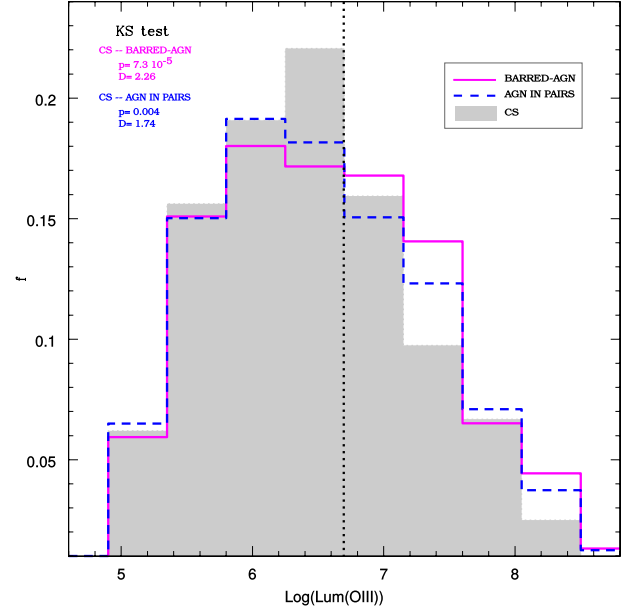
Fig. 3. Distribution of \log(Lum[\text{OIII}]) for barred AGN galaxies (solid line), AGNs in pair systems (dashed line) and unbarred AGNs in the control sample (full surfaces). The D and p -values of the KS test between both samples (BARRED-AGN, AGN IN PAIRS) and the CS is inset in the upper-left corner of the figure. The dotted vertical line represents the excess of Lum[\text{OIII}] for the BARRED-AGN.
