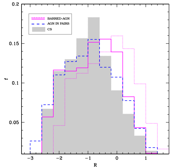
Fig. 4. Distribution of accretion rate parameter, \mathcal{R} = \log(Lum[\text{OIII}]/M_{\text{BH}}) , for barred AGN galaxies (dotted line), AGNs in pair systems (dashed line), and unbarred AGNs in the control sample (full surfaces). The solid line represents the \mathcal{R} distribution for barred AGN galaxies, using the same parameters, \alpha and \beta , as for the unbarred galaxies to calculate M_{\text{BH}} (see Eq. (2)).
