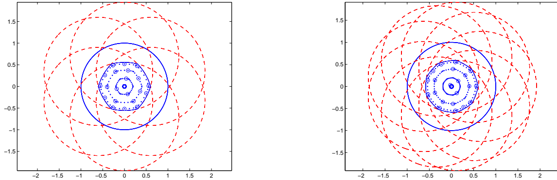
Figure 4: Quadrature nodes for two diaphragms, degree n = 5 ; Left: 6-blade diaphragm, aperture 0.6, blade curvature 0.8, 28 \times 6 = 168 nodes (·) compressed by QR with column pivoting into 21 (○); Right: 9-blade diaphragm, aperture 0.8, blade curvature 0.8, 28 \times 9 = 252 nodes compressed by NNLS into 21.
