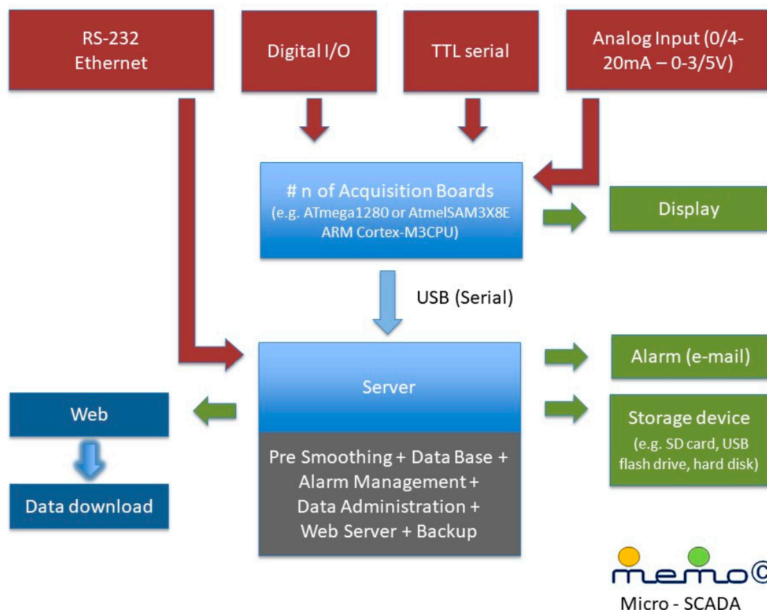
Figure 2. MEMO micro-supervisory control and data acquisition (SCADA).
