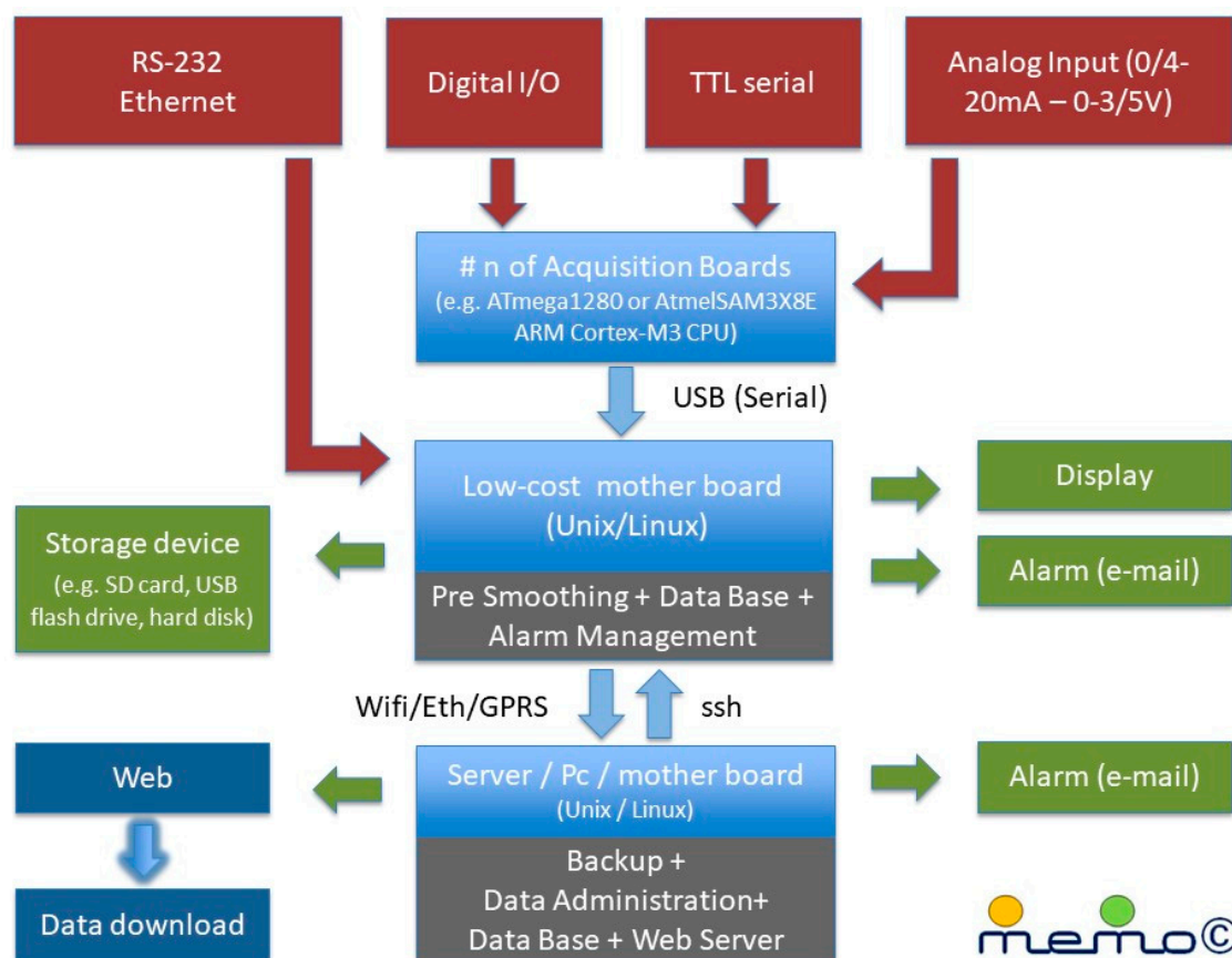
Figure 1. MEMO general architecture.
