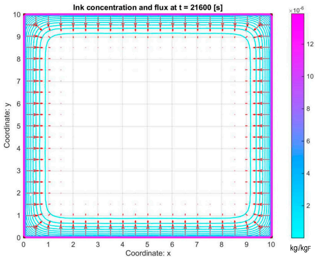
Figure 6. Migration of isopropylthioxanthone through polyethylene (PE) packaging—isoconcentration profiles in milk with 2D model.
