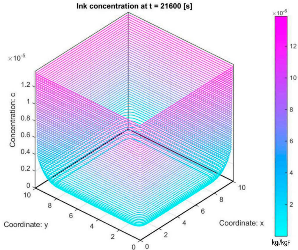
Figure 7. Migration of isopropylthioxanthone through PE packaging—isoconcentration profiles in milk with 3D model.
