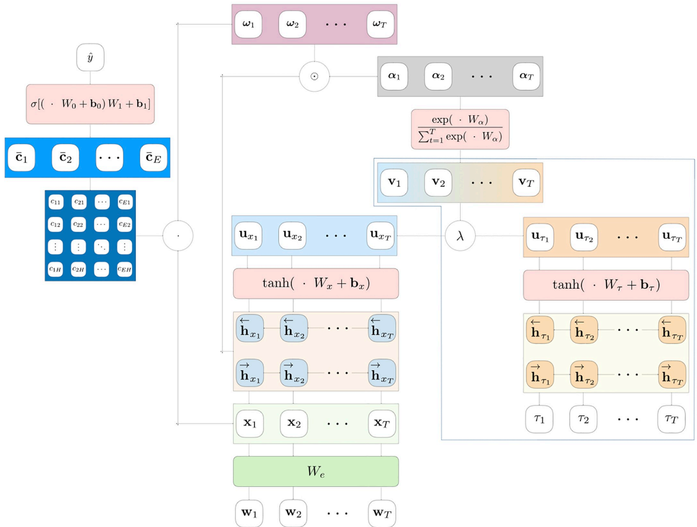
Fig 2. Neural attention model. A visual representation of the attention mechanism for sequences classification. When \lambda = 1 this corresponds to a standard bidirectional attention model, whereas when \lambda \neq 1 the time span sequence \tau_1, \dots, \tau_T can guide the model to focus on the most relevant elements of the sequence. We call Tangle the case in which the value of \lambda is jointly learned during the training process. A blue dashed line highlights the timestamps attention guiding mechanism.
