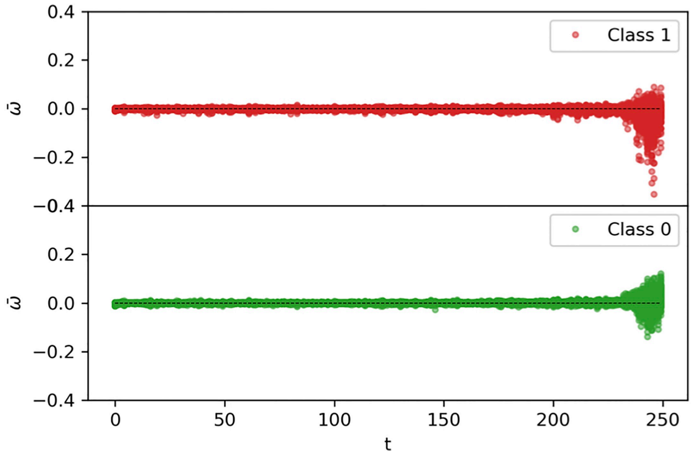
Fig 6. Attention contribution. Manhattan plot of the attention contribution \omega estimated by Tangle on the test set. As we can see, the model correctly focuses its attention on the most recent claims, which have nonzero contributions. From this plot we can also appreciate the different representations learned for the two classes.
