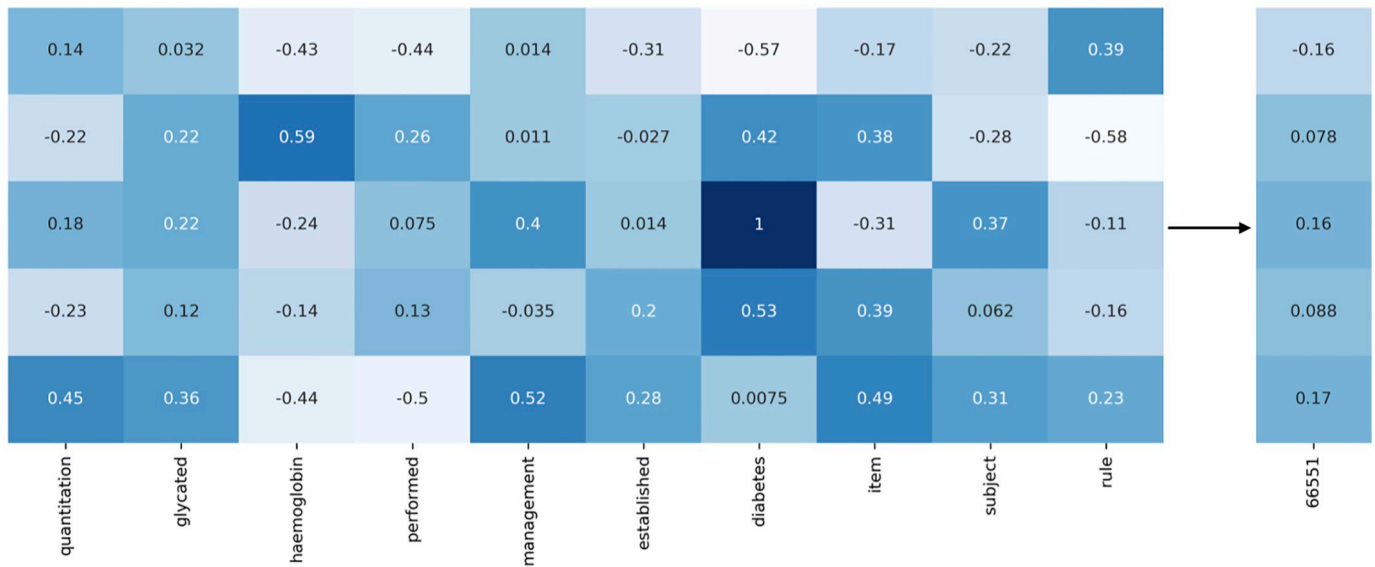
Fig 3. MBS item embedding. A schematic representation of our word embedding strategy to achieve meaningful representations of MBS items. Here, we consider a 10-words textual representation of the MBS item no. 66551. To each word is associated the corresponding word-embedding, which, in this picture, is a 5-dimensional vector to guarantee readability. The final representation of the considered item is achieved by averaging.
