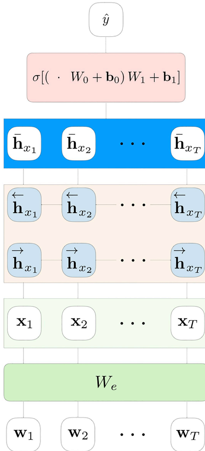
Fig 1. LSTM for sequence classification. A visual representation of a simple bidirectional LSTM for sequences classification. This architecture is used in this work for the sake of comparison, and it is referred to as baseline . In this work we adopted LSTM recurrent cells, in order to exploit their ability to learn long-time relationship in the sequences. However, similar architectures can be devised with vanilla RNN, Gated Recurrent Units (GRU) [17] or other types of temporal architectures.
