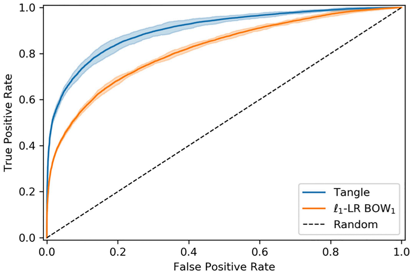
Fig 4. Average ROC curves. ROC curves obtained averaging the 10 Monte Carlo cross-validation iterations for best and worst method: i.e. Tangle and \ell_1 -LR 1-BOW respectively. Shaded area corresponds to \pm 3\sigma , where \sigma is the standard deviation. For ease of readability, only ROC curves corresponding to best and worst performing models are shown.
