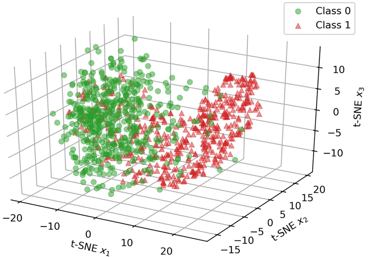
Fig 5. t-SNE embedding. 3D scatter-plot of a random extraction of 500 samples projected on a low-dimensional embedding, estimated by t-SNE [30], from the sample representation learned by Tangle. Samples belonging to the two classes, represented with green circles and red triangles, can be seen as slightly overlapping clusters.
