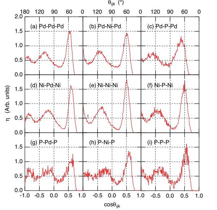
FIG. 5. (Color online.) Selected partial bond angle distributions \eta(\cos \theta_{ijk}) . The \theta_{ijk} values are given at the top of the figures.
