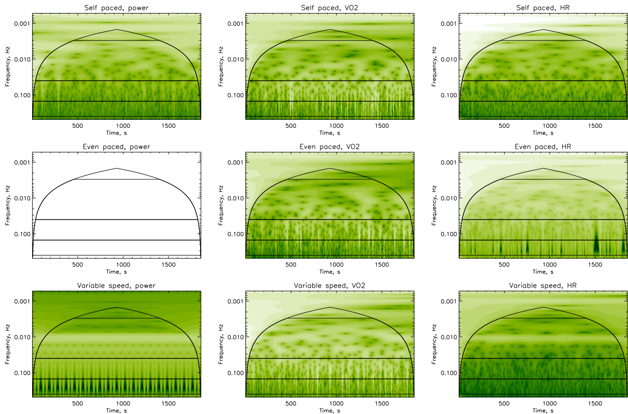
FIGURE 4: Wavelet logarithmic power maps for the studied signals. Three rows correspond to the different trial regimes. The columns represent different quantities measured in the study. The curve in each of the plots identifies the cone of influence, above which the displayed power values are affected by the boundary effects. These regions are excluded from the mean power calculations. The horizontal lines represent the frequencies separating the bands, as given in Table 1.
