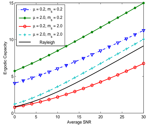
Fig. 1: Ergodic capacity versus average SNR under \kappa - \mu / inverse gamma fading channels for \kappa = 1 and different values of \mu , and m_s .
