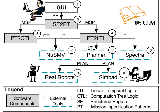
Figure 2: Components of the PsALM toolchain.
