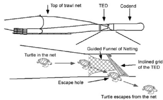
Figure 1. Diagrammatic representation of a Turtle Excluder Device fitted to a trawl net http://www2.dpi.qld.gov.au/fishweb/10559.html
