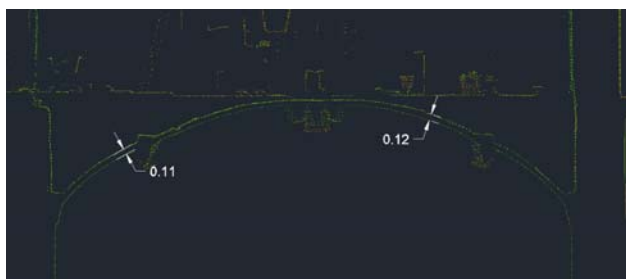
Figure 15: Point cloud section during the restoration works. The measure of the vault section can be obtained.
