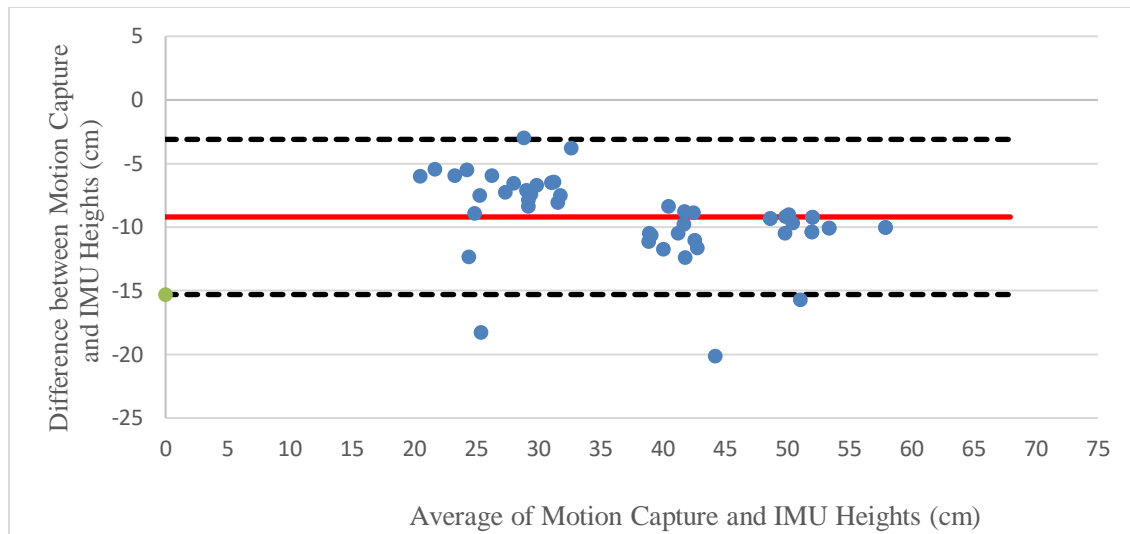
Figure 6. Bland-Altman plot of in-lab heights for trampoline straight jumps with average difference and limits of agreement.
