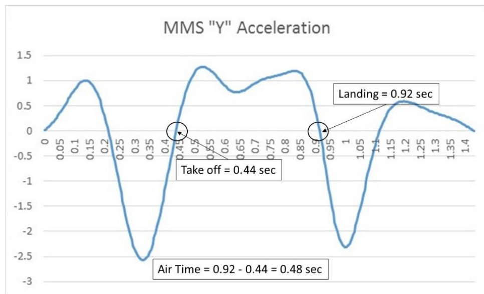
Figure 3. Typical MMS acceleration signal from a jump in the laboratory showing the Take-off and Landing times and the calculation of the Airtime.
