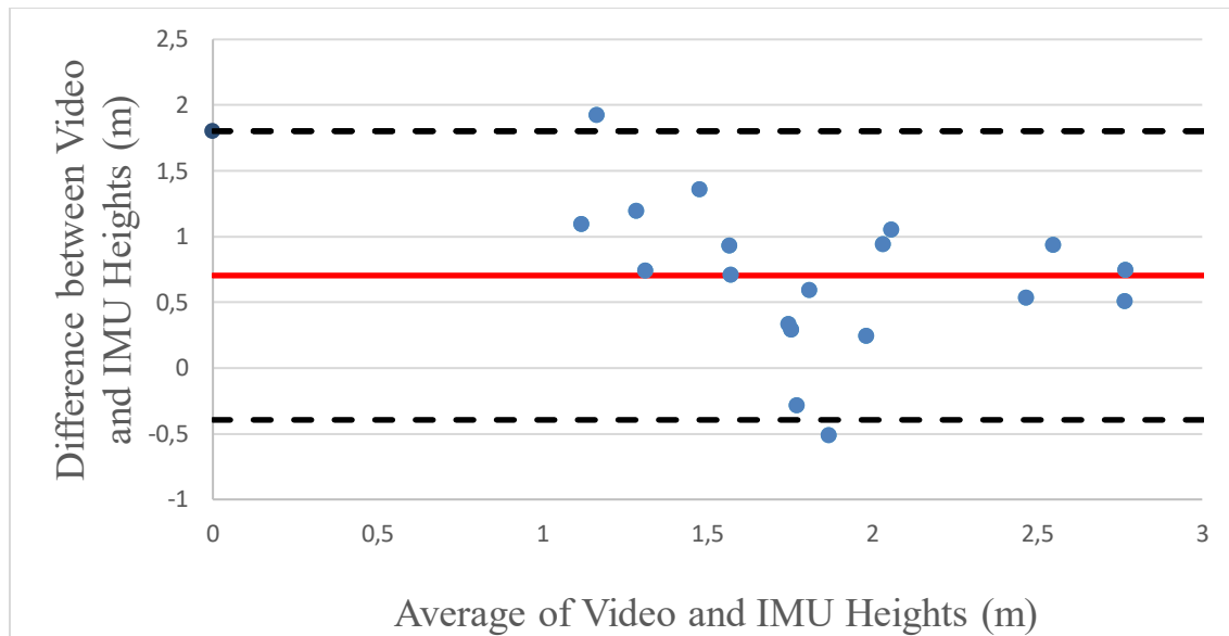
Figure 5. Bland-Altman Plot with average difference between video and IMU heights for All Conditions. The dashed line represents the limits of agreement and the straight line is the average difference.
