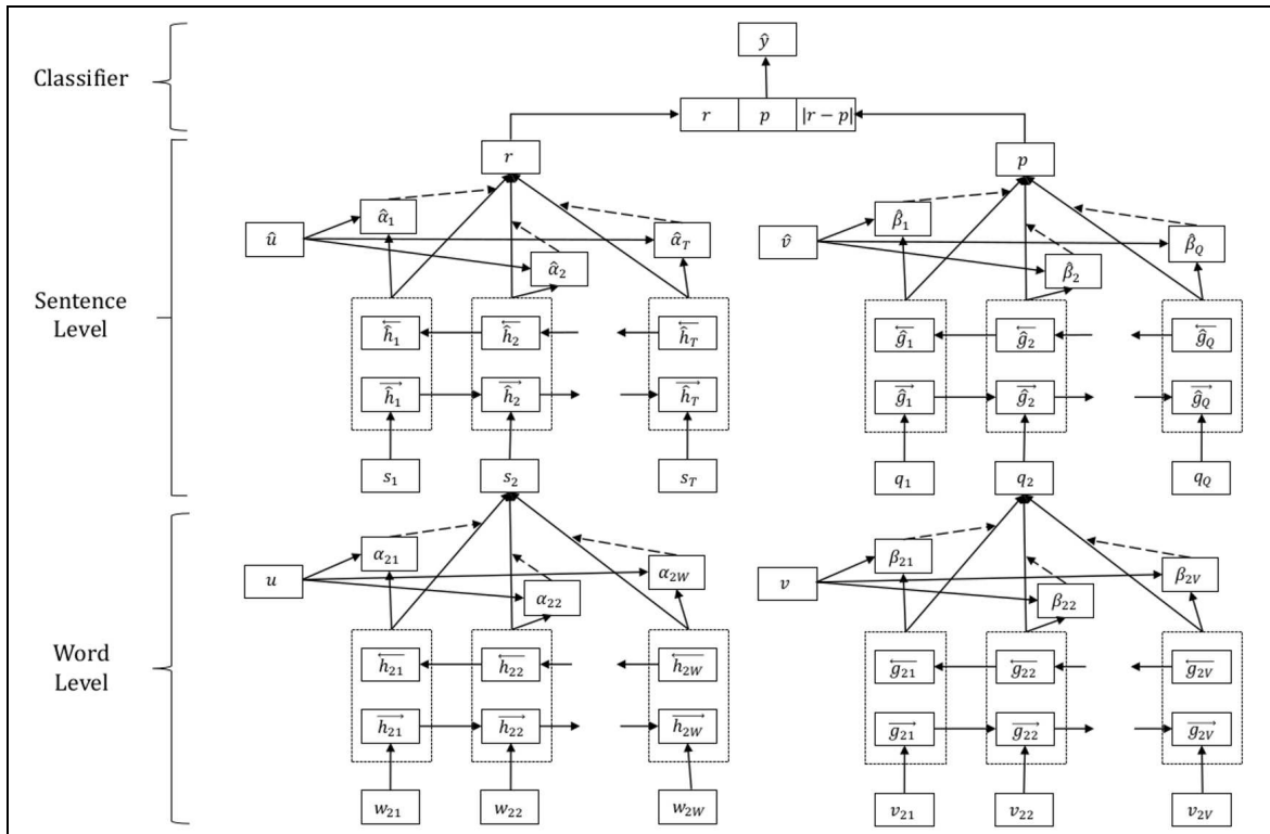
Figure 1: SHA-NN architecture proposed in (González et al., 2019)
