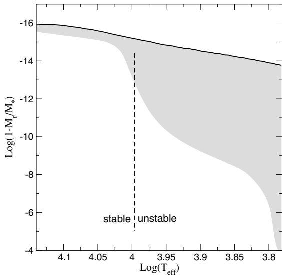
Figure 14. Location of the convection zone as given by the outer mass fraction as a function of effective temperature (grey domain). The vertical, dashed line indicates the value of effective temperature below which g -modes become unstable. The thick line marks the outer edge of the convection zone which is near the location of the photosphere.
