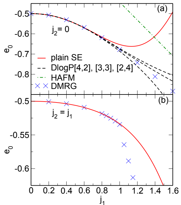
Figure 4: (a) Comparison between e_0 from plain SE (red solid lines) with DMRG for L = 30 and m = 300 (blue crosses), along j_2 = 0 . Black dashed lines refer to three DlogPadé approximants to eqn. (7). For reference the ground state energy of the 1D HAFM is also depicted (green dash-dotted). (b) Comparison of plain SE (red solid lines) with DMRG (blue crosses) along j_1 = j_2 . Up to the first-order transition discussed in section II, the agreement is excellent.
