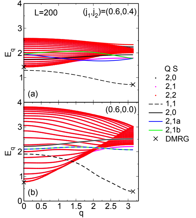
Figure 8: Momentum resolved spectrum of all states on the FFST with Q \leq 2 for (j_1, j_2) = (0.6, 0.4) and (0.6, 0.0) . Apart from four genuine one-particle states, i.e. three triplets (black dashed, blue solid, green solid), and one singlet (black solid), there are three two-particle continua with S=0,1,2 , and three collective two-particle states: a bound triplet (magenta dots), an anti-bound singlet (black dots) and an anti-bound quintet (red dots). Only \sim 10\% of the scattering states between the lower and upper bounds of the continua are depicted to avoid graphic cluttering. DMRG results for one and two-particle states at zone-boundaries(centers) are depicted with large crosses.
