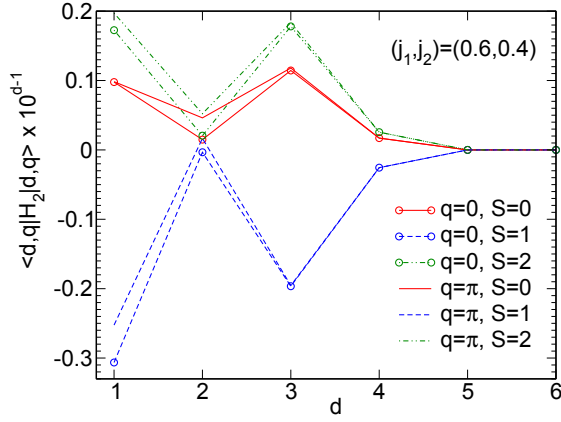
Figure 7: Diagonal element of the irreducible interaction \langle q, d | H_2 | q, d \rangle versus relative distance of two particles for S = 0, 1, 2 , and for q = 0 and \pi , multiplied by 10^{d-1} . (The matrix elements of H_2 at O(6) are zero for d = 5, 6 .)
