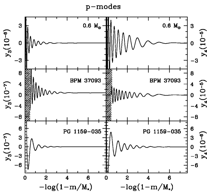
Fig. 3. Same as Fig. 1 for the p -modes of our 0.6 M_\odot fiducial model, for BPM 37093 and for PG 1159-035.
