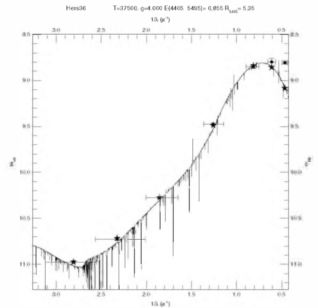
Figure 2. UBVIJHK_s photometry (data with error bars), SED corresponding to the best CHORIZOS fit (spectrum) and synthetic photometry associated with the best SED (stars) for Her 36. For the photometry, vertical error bars display photometric uncertainties and horizontal ones display the approximate extent of the passband. The H and K_s filters were not used for the CHORIZOS fit because of the infrared excess of Her 36, which is readily apparent in the plot.
