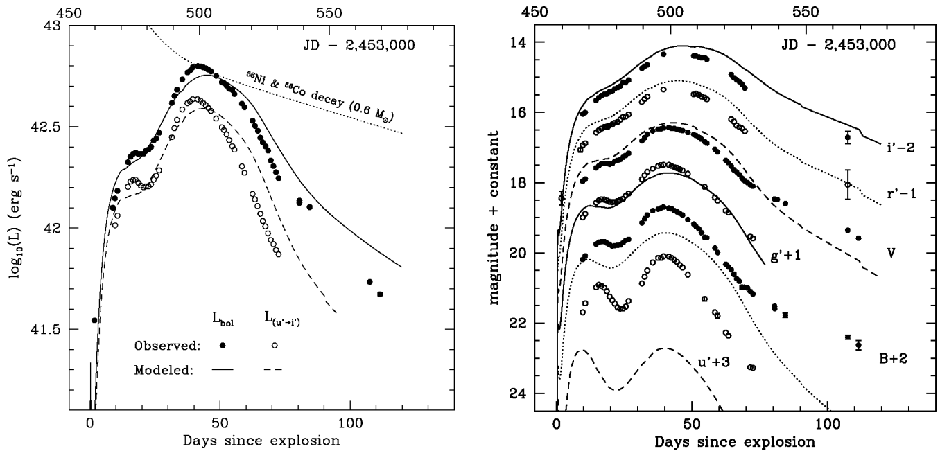
FIG. 10.— Left : Modeled bolometric (solid line) and UVOIR (dashed line) luminosities of the mixed 8.29 M_{\odot} WN star explosion. The circles mark the UVOIR luminosity L_{u' \rightarrow i'} (open) and the bolometric luminosity L_{\text{bol}} (closed), as derived from the observations. The dotted line shows the predicted luminosity if the ejecta were able to trap the entire \gamma -ray output of 0.6 M_{\odot} of radioactive ^{56}\text{Ni} produced in the explosion. The time of outburst was assumed to be JD 2,453,458. Right : Modeled u'g'r'i'BV light curves (lines) compared with the observations (circles).
