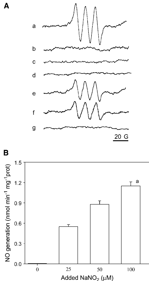
Figure 2. Nitrite-dependent NO generation. A, EPR spectra of the (MGD) 2 -Fe(II)-NO adduct. a, Chloroplasts were incubated for 3 min in the presence of MGD-Fe (10:1 mM) and 1 mM NaNO 2 . b, Boiled chloroplasts were incubated under the conditions indicated above. c, Chloroplasts were incubated for 3 min in the presence of the spin trap solution and 1 mM NaNO 3 . d, Isolation buffer was incubated for 3 min in the presence of MGD-Fe (10:1 mM) and 1 mM NaNO 2 . e, Chloroplasts were incubated for 3 min in the presence of MGD-Fe (10:1 mM), 1 mM NaNO 2 , and 1 μM DCMU. f, Thylakoids were incubated for 3 min in the presence of MGD-Fe (10:1 mM) and 1 mM NaNO 2 . g, Stroma were incubated for 3 min in the presence of MGD-Fe (10:1 mM) and 1 mM NaNO 2 . B, Nitrite-dependent NO generation in isolated chloroplasts in the presence of NaNO 2 up to 100 μM. Quantification was performed by double integration of the EPR signals. Data are expressed as means ± SE of six independent experiments with two replicates in each experiment. Superscript a, Significantly different from values for isolated chloroplasts incubated in the presence of 25 μM NaNO 2 ; P \leq 0.05 (Statview for Windows Version 5.0; SAS Institute).
