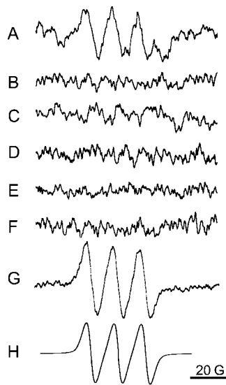
Figure 1. Arg-dependent NO generation. A to H, EPR spectra of the (MGD) 2 -Fe(II)-NO adduct from chloroplasts incubated for 10 min in the presence of MGD-Fe (10:1 mM), 1 mM Arg, 1 mM CaCl 2 , 5 mM MgCl 2 , and 0.1 mM NADPH (A); previously boiled chloroplasts were incubated under the conditions indicated above (B); chloroplasts were incubated under the conditions indicated above in the absence of NADPH (C); the reaction medium indicated above incubated in the absence of chloroplasts (D); chloroplasts incubated for 10 min simultaneously with 5 mM L-NAME or L-NNA and all the substrates indicated above (E and F); 50 μM GSNO and 50 μM DTT incubated 10 min in the presence of MGD-Fe (10:1 mM; G); and computer-simulated spectrum employing the following spectral parameters: g = 2.03 and a_N = 12.5 G (H). Measurements were performed at room temperature and four scans, except for GSNO (one scan).
