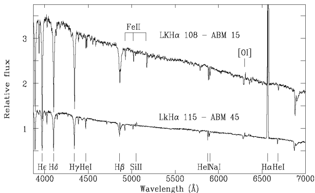
Figure 2. Flux-calibrated spectra of the two Herbig Ae/Be stars observed in M8. The rest-wavelengths of the most prominent lines, including the Balmer series ( He\epsilon , H\delta , H\gamma , H\beta , H\alpha ), the Fe II (42) multiplet, He I ( \lambda\lambda 4471, \lambda 5876 and \lambda 6678 ) and Na I \lambda\lambda 5890, 5896 lines, are indicated. The high S/N ratio of these spectra allowed us to detect new spectral emission features, such as Si II \lambda\lambda 5041, 5056 and \lambda\lambda 6347, 6371 and [O I] \lambda\lambda 6300, 6364 , which are also marked in the figure.
