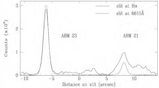
Figure 7. Cuts of the slit along the position of the H \alpha line (solid line) and the continuum at 6615 \text{ \AA} (dashed line). In order to compare the two spectra, a quadratic fit of the background was subtracted from both of them.
