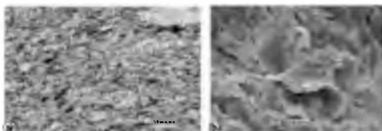
Fig 11 Micrographs of the C/S Facies La Siempre Verde quarry (a) Thin section Illitic clay (2M 1 and 1M 1 , polytypes) bearing rutile needles in a sagenite-like texture (b) Scanning electron micrograph of illitic clays showing face-to-face disposition of platelets, certain swirl pattern and rugged borders
