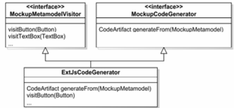
Fig. 8.b. Code generator structure
