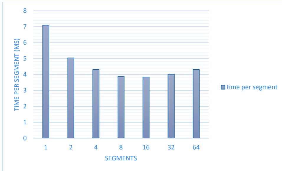
Figure 36. Performance effect of creature with more segments. Displays time divided by amount of segments.
