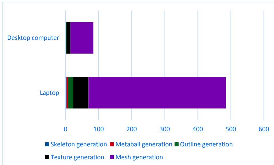
Figure 31. Time taken by individual steps (ms).
