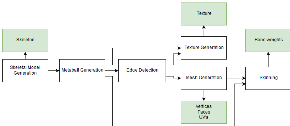
Figure 10. Steps of the developed generation process, green signifies final outputs, arrows indicate data flow.
