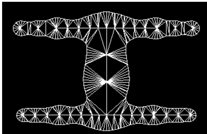
Figure 21. Example of triangulation using outline and metaball locations.
