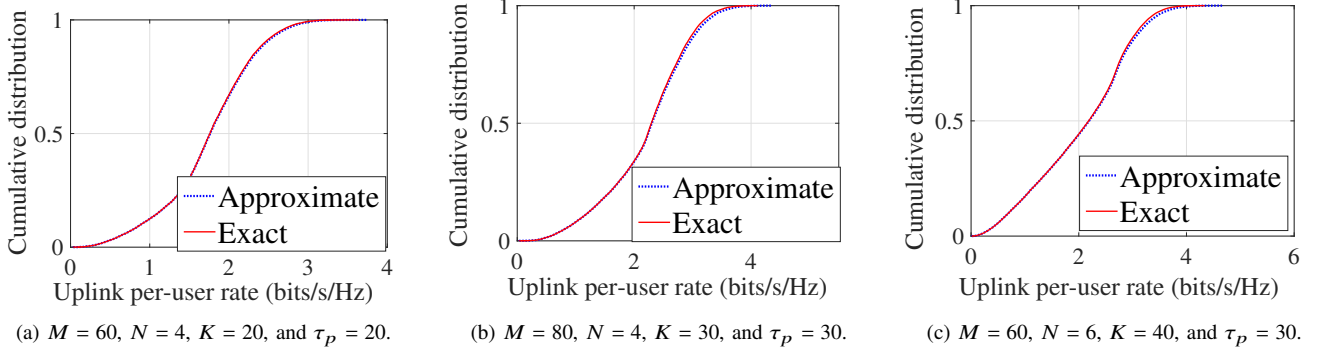
Figure 11. Uplink per-user rate of cell-free Massive MIMO with. Here, the term ‘‘Exact’’ refers to the case where we use the exact result (50), whereas the term ‘‘Approximate’’ refers to the case where we use the approximation (52). In all figures, we set \alpha = 2 quantization bits, and use equal power allocation.
