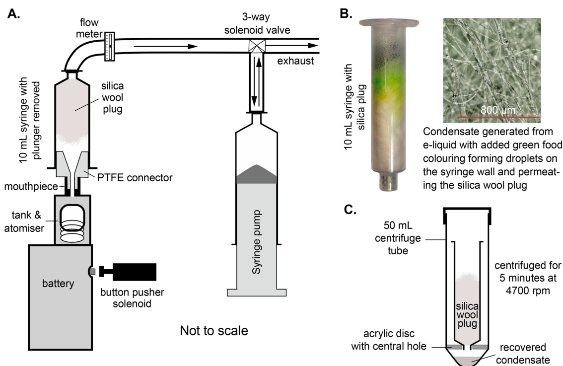
Figure 1. Schematic outline of vapor collection and recovery. A: Power to the atomizer is synchronized with the inhalation cycle of a syringe pump (electronics omitted for simplicity). The aerosol is drawn via the mouthpiece into the open end of a 10 mL syringe packed with a plug of silica wool which traps the particulate fraction. B: Silica wool plug contained in syringe after 50 puffs of vaping an e-liquid spiked with green food coloring. Enlargement shows condensed aerosol droplets on the syringe walls and silica strands of the plug. C: Liquid condensate is recovered by centrifuging the syringe containing the silica wool within a 50 mL centrifuge tube centered on a hole in an acrylic disc located above the tapering end of the tube where separated liquid collects.
