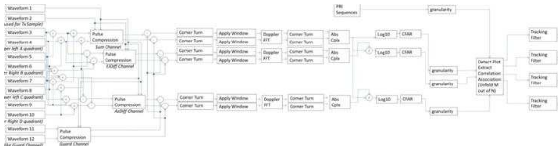
Figure 9. Signal and processing block diagram
