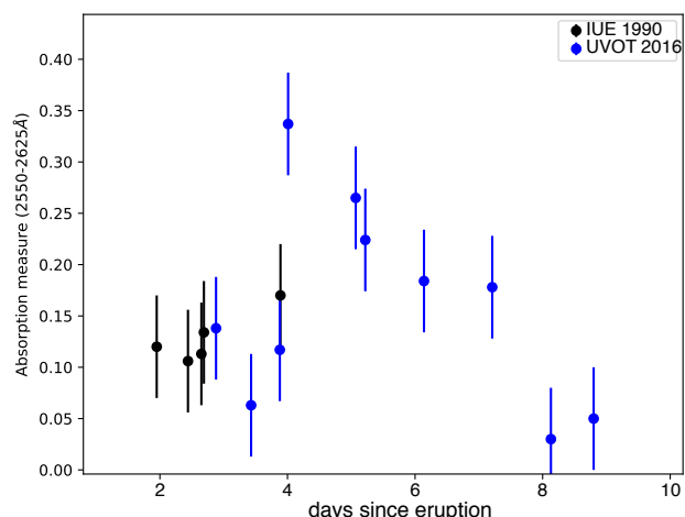
Figure 14. The relative absorption below the continuum of the region 2550\text{--}2625 \text{ \AA} which includes the Fe II 2600 \text{ \AA} resonance line. At day 4 a recombination wave occurs.
