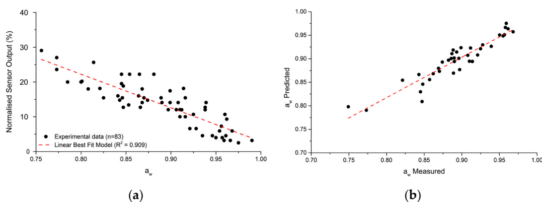
Figure 2. (a) Correlation between the a_w and normalized sensor output at selected frequencies. PLS regression (b) shows the capability of the sensor in terms of measured vs. predicted aw values.
