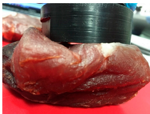
Figure 3. Uneven surfaces, which are more prevalent as the product dries and hardens, introduce gaps between the sensitive surface of the microwave probe and the sample.
