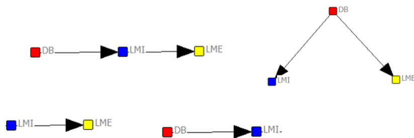
Figure 2. Path analysis of ego networks
