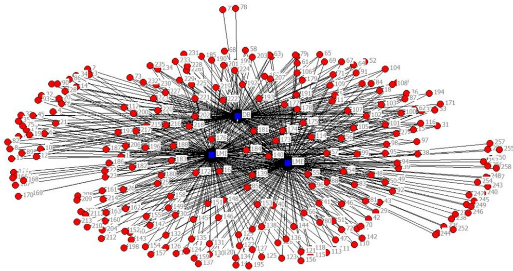
Figure 1. Measures of centrality of a complete network
