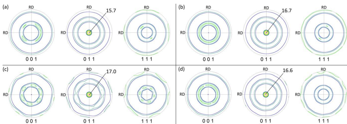
Figure 2. Pole figures of the samples with unimodal grain size distribution in the (a) as-received and annealed at (b) 1300, (c) 1600 and (d) 1900 °C conditions. DA perpendicular to the paper. RD: radial direction. Intensity levels: 1-2-4-6-8-11-16 times random.
