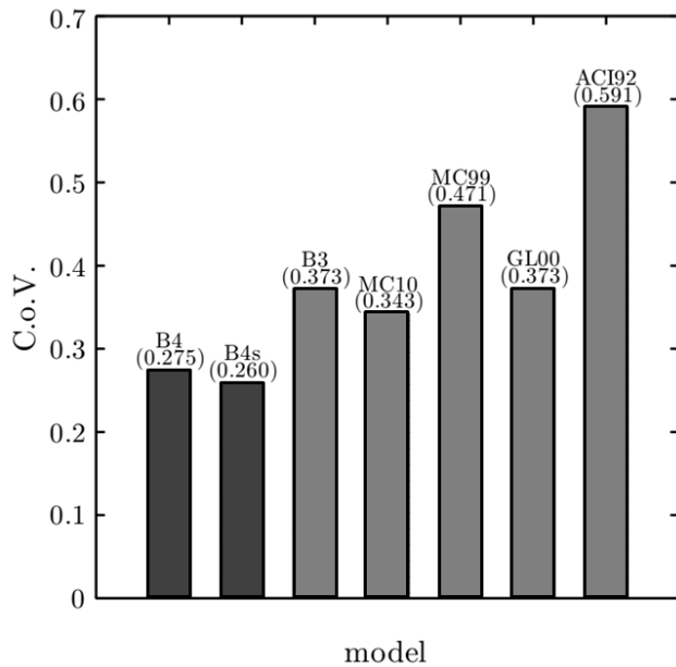
Figure 6. Comparison of creep models based on full laboratory database and bridge bridge deflection data
