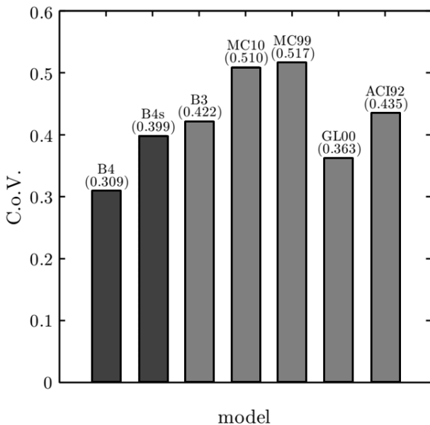
Figure 7. Comparison of shrinkage models based on full laboratory database
