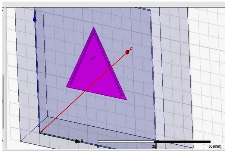
Figure 9: Design of SIW based Equilateral Triangular Micro strip Antenna in HFSS Workspace.
