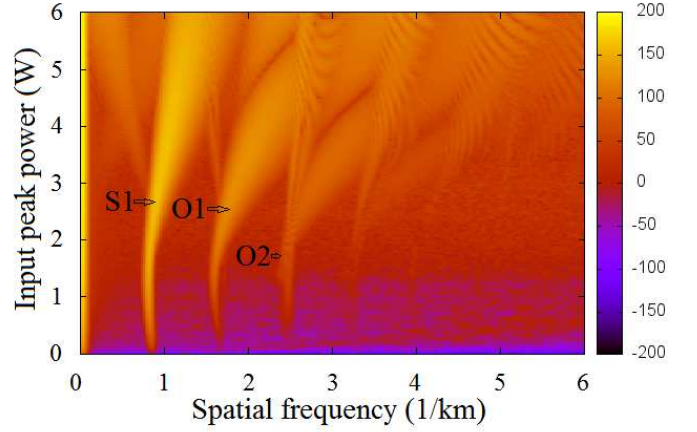
Figure 7: Power spectrum for different values of input power P_0 , laser frequency separation LFS = 100 \text{ GHz} , group-velocity dispersion parameter \beta_2 = -15 \frac{\text{ps}^2}{\text{km}} , the nonlinear coefficient \gamma = 2 \text{ W}^{-1}\text{km}^{-1} , and optical losses \alpha = 0.05 \frac{\text{dB}}{\text{km}}
