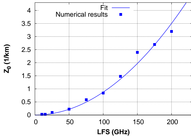
Figure 4: Fundamental frequency Z_0 depending on the laser frequency separation LFS
