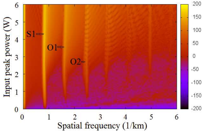
Figure 8: Power spectrum for different values of input power P_0 , laser frequency separation LFS = 100 \text{ GHz} , group-velocity dispersion parameter \beta_2 = -15 \frac{\text{ps}^2}{\text{km}} , the nonlinear coefficient \gamma = 2 \text{ W}^{-1}\text{km}^{-1} , and optical losses \alpha = 0.2 \frac{\text{dB}}{\text{km}}
