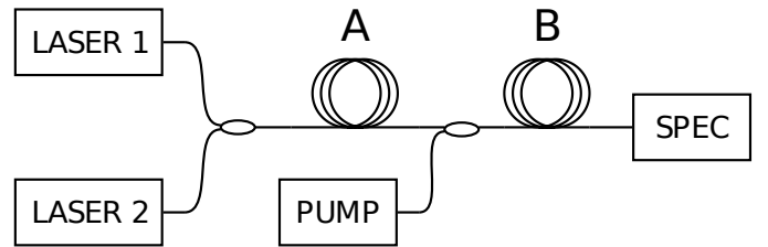
Figure 1: Schematic representation of the proposed approach for generation of optical frequency combs. LASER 1: fixed CW laser, LASER 2: tuneable CW laser, A: conventional single-mode fibre, B: Er-doped fibre, PUMP: pump laser for B, SPEC: astronomical spectrograph [26]
