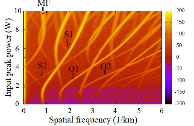
Figure 3: Power spectrum for different values of input power P_0 , laser frequency separation LFS = 100 GHz, group-velocity dispersion parameter \beta_2 = -15 \frac{\text{ps}^2}{\text{km}} , and the nonlinear coefficient \gamma = 2 \text{ W}^{-1}\text{km}^{-1}
