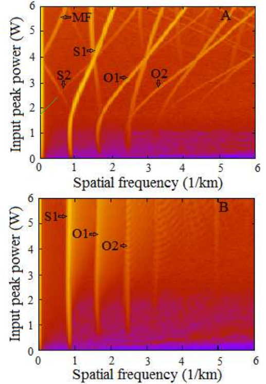
Figure 9: Power spectrum for different values of input power P_0 , laser frequency separation LFS = 100 GHz, group-velocity dispersion parameter \beta_2 = -15 \frac{\text{ps}^2}{\text{km}} , the nonlinear coefficient \gamma = 2 \text{ W}^{-1}\text{km}^{-1} , and optical losses \alpha = 0 \frac{\text{dB}}{\text{km}} (A) \alpha = 0.2 \frac{\text{dB}}{\text{km}} (B)
