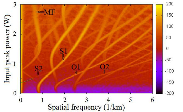
Figure 6: Power spectrum for different values of input power P_0 , laser frequency separation LFS = 100 \text{ GHz} , group-velocity dispersion parameter \beta_2 = -15 \frac{\text{ps}^2}{\text{km}} , and the nonlinear coefficient \gamma = 10 \text{ W}^{-1}\text{km}^{-1}
