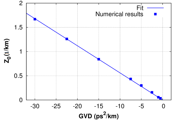
Figure 5: Fundamental frequency Z_0 depending on the GVD parameter \beta_2
