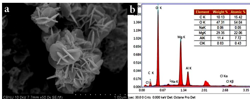
Fig. 2. SEM image of Mg/Al LDH and their EDX results.
