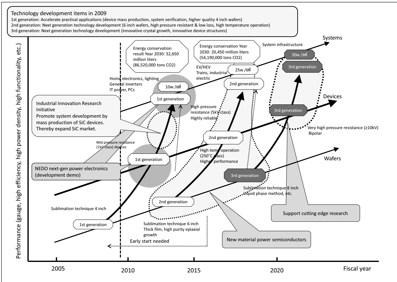
Figure 5 : SiC Power Semiconductor Road Map
