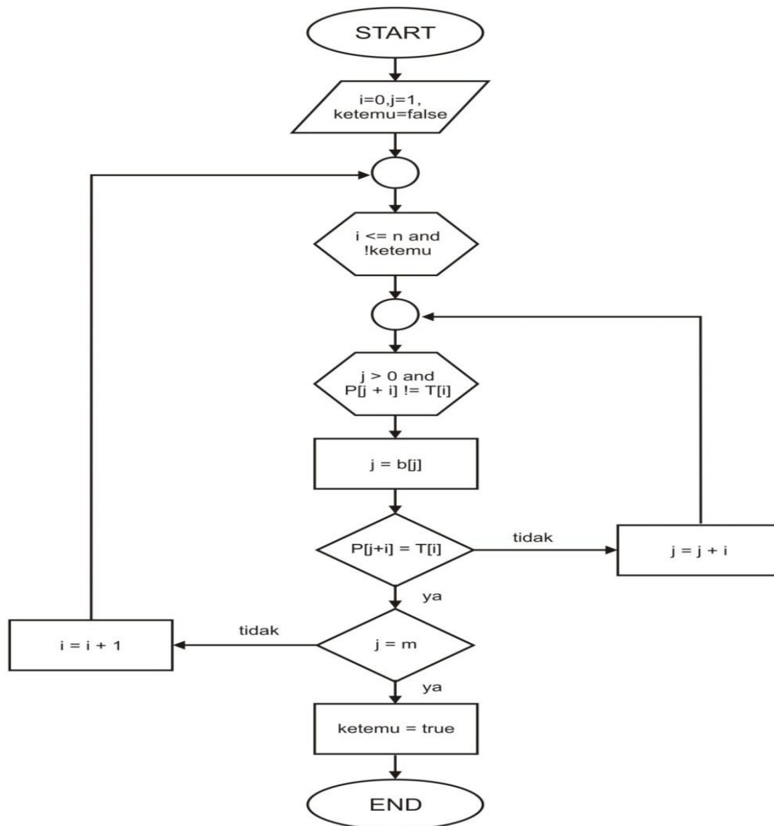
Gambar 24. Flowchart Algoritma Knuth-Morris-Pratt
