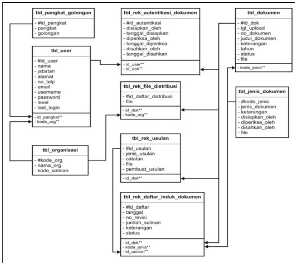
Gambar 7. Logical Record Structure
