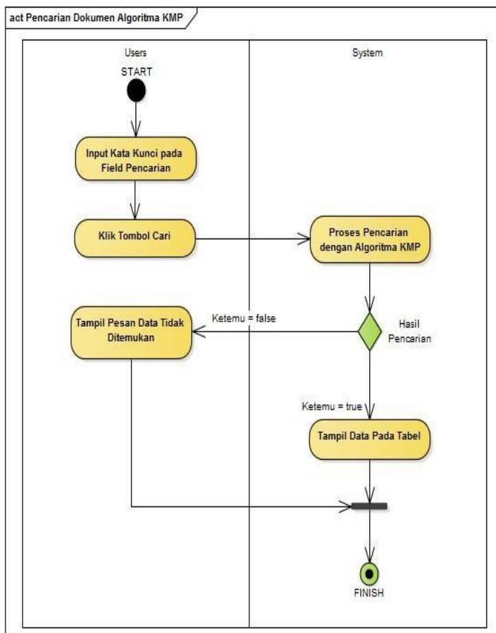
Gambar 11. Activity Diagram Pencarian Data Algoritma KMP
