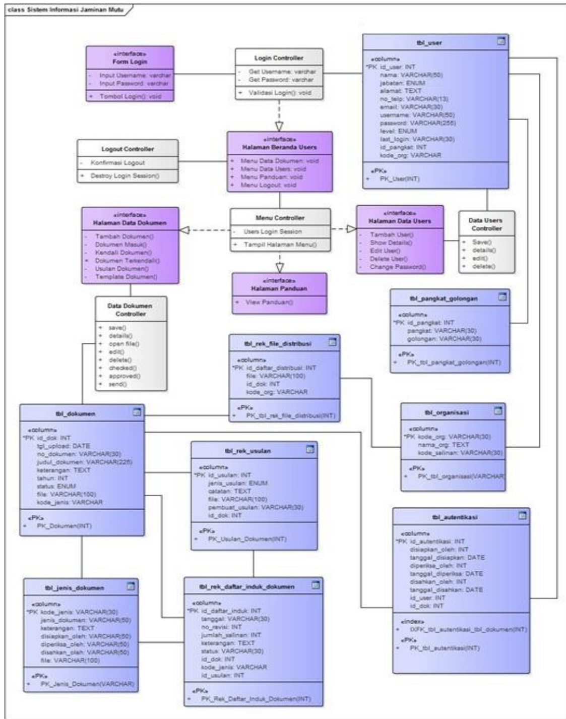
Gambar 23. Class Diagram
