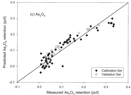
FIG. 5. Relationship between measured values of: (a) CuO, (b) CrO_3 , and (c) As_2O_5 retentions and those predicted by PLS-2 modeling using NIR spectra for CCA samples.
