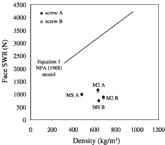
FIG. 1. Predicted change in face SWR with board density from NPA (1968) and converted to SI units. Average values for MS and M2 grade particleboard from press lines A and B are shown for comparison.
