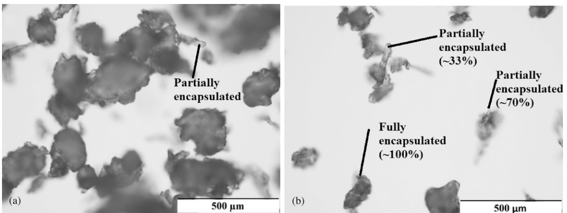
Figure 2. Optical microscope images of encapsulated cellulose particles by wax and surfactants with different ratios: (a) 8:2 and (b) 7:3.
