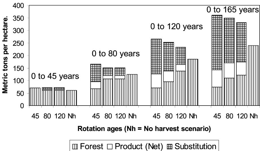
Fig. 3. Average annual carbon in forest, product, and concrete substitution pools for different rotations and specified intervals.
