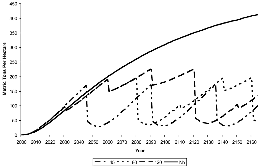
Fig. 1. Carbon in forest pools for different rotations.
